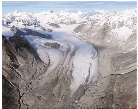
© US Geological Survey/R. March.
