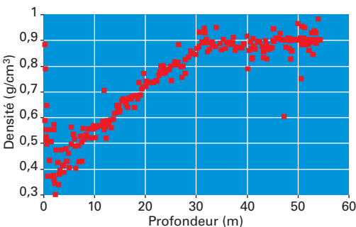
Source : Great Ice, IRD.
