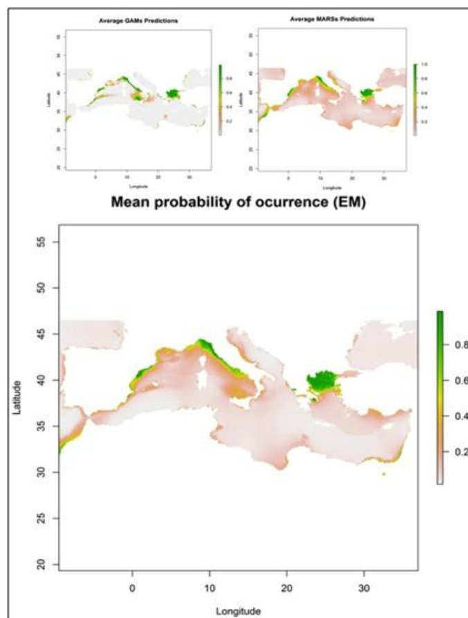
Figure 2. Suitable habitats for Mnemiopsis leidyi . Average prediction from GAM (upper-left panel) and MARS models (upper-right panel). Lower panel shows the ensemble forecasting for the potential distribution of M. leidyi in the Mediterranean Sea (Canepa et al. , 2013).
