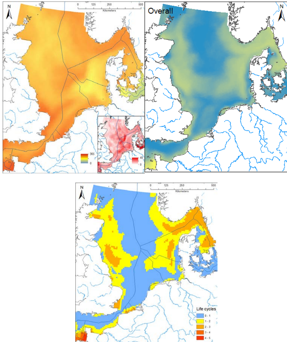
Figure 1. Maps showing the average (for 2005–2011) number of days per year suitable for survival of Mnemiopsis leidyi (top left) and reproduction (top right) as determined by temperature, salinity and adult food (mesozooplankton); and the number of reproductive cycles (bottom left) possible within the time window when conditions are suitable for Mnemiopsis leidyi reproduction, assuming a life cycle length of 40 days, as at 15°C.
