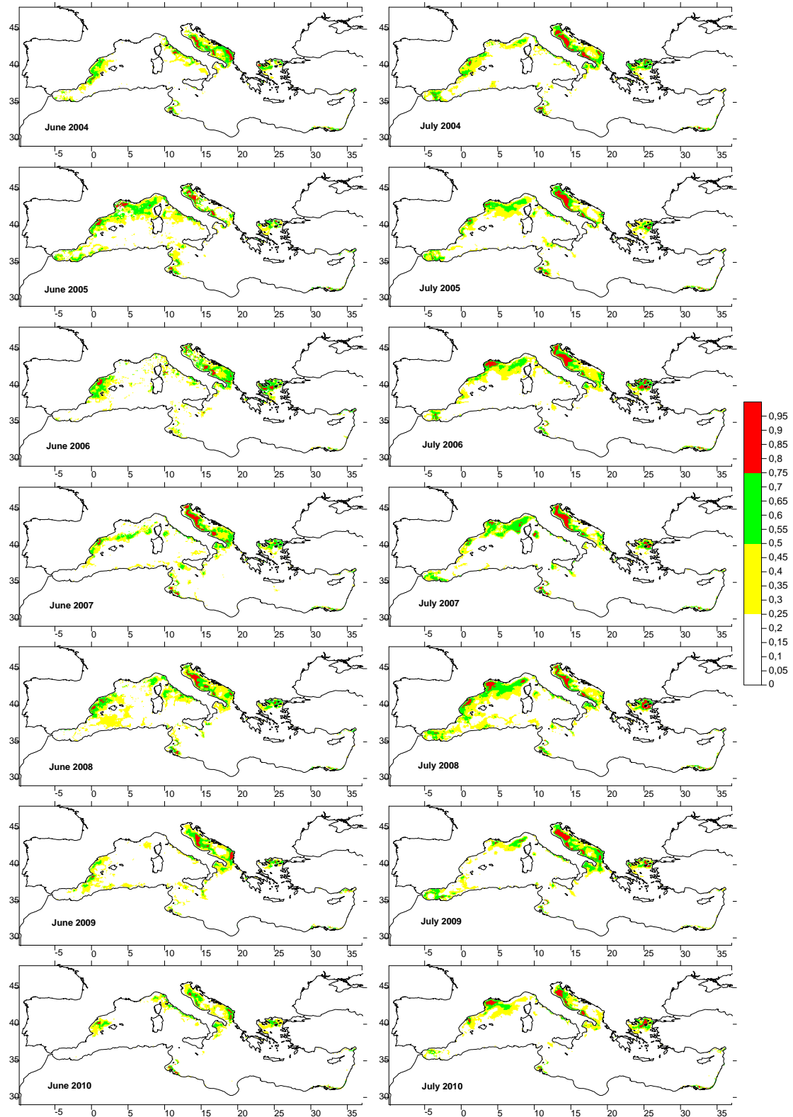
Figure 3. Maps of the probability for M. leidyi potential presence in the Mediterranean basin, based on maximum entropy modelling from June 2004–2010 (left) and July 2004–2010 (right).
