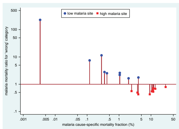
Fig. 3. Sensitivity analysis showing the effect of choosing the ‘wrong’ malaria endemicity setting (‘high’ and ‘low’ reversed) in processing VA data using the InterVA-4 model, by site.
