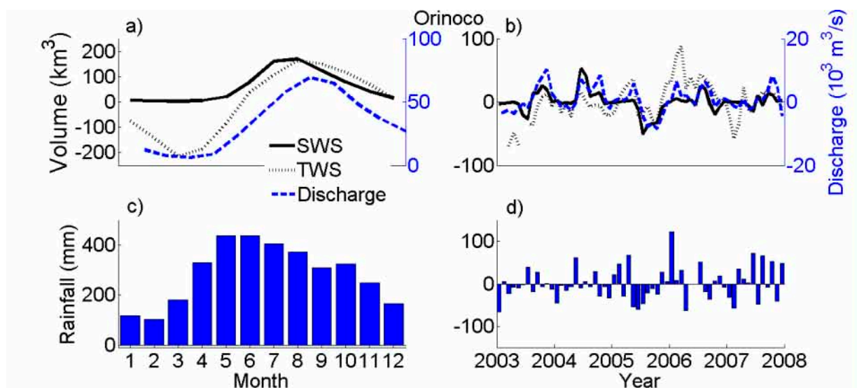
Figure 9. (a) Annual cycles and (b) deseasonalized variations of surface water storage (SWS) from altimetry and imagery (black line), the total water storage (TWS) anomaly from GRACE regional solutions in the Orinoco Basin (dotted black line) and discharge at Ciudad Bolivar (dashed blue line). (c) Annual cycle and (d) deseasonalized variations of rainfall TRMM 3B43 v7 over 2003–2007.
