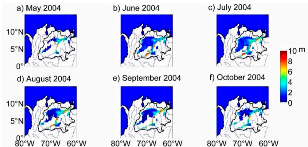
Figure 6. Monthly maps of water levels from altimetry spatially extended with GIEMS for (a) May, (b) June, (c) July, (d) August, (e) September and (f) October 2004.
