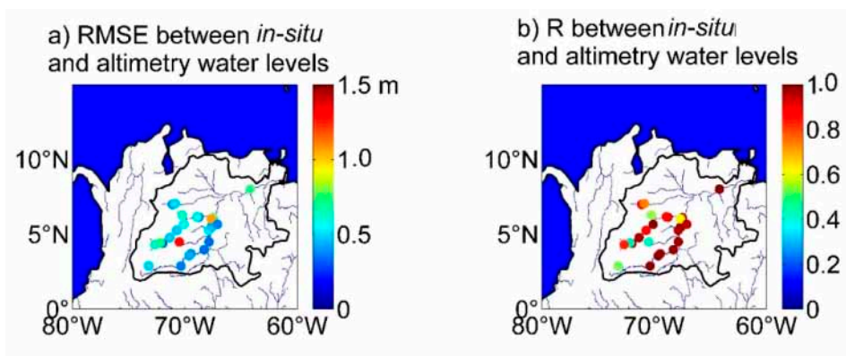
Figure 4. Comparisons between altimetry-based and in situ water levels over the Orinoco Basin. (a) RMSE (m), (b) R.
