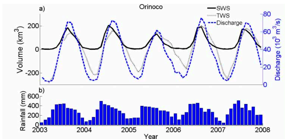
Figure 8. Time series of (a) surface water storage (SWS) from altimetry and imagery (black line), the total water storage (TWS) anomaly from Gravity Recovery and Climate Experiment (GRACE) regional solutions in the Orinoco Basin (dotted black line) and discharge at Ciudad Bolivar (dashed blue line); (b) rainfall from TRMM 3B43 v7 over 2003–2007.
