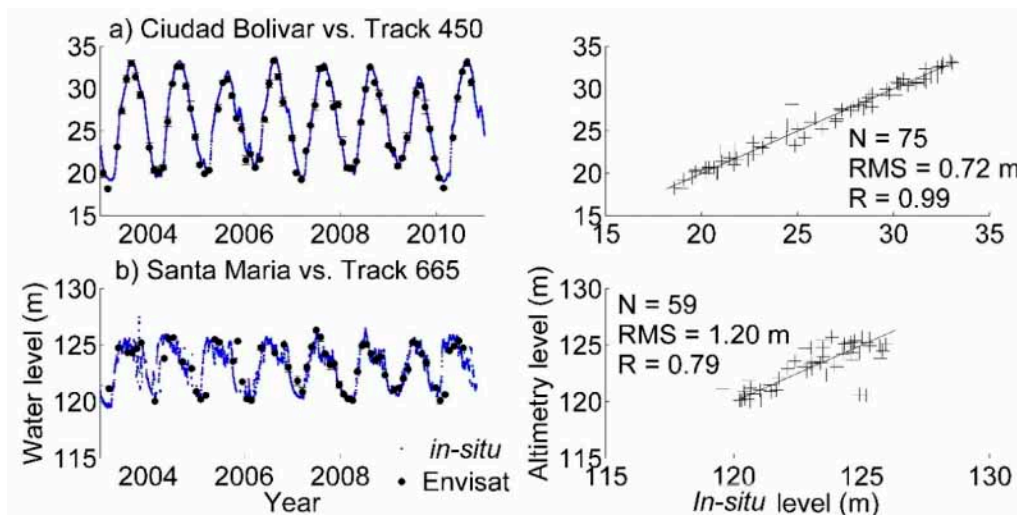
Figure 3. Two examples of water levels derived from Envisat radar altimetry and compared with in situ gauge records over 2003–2010. (a) Track 450 at ~74 km upstream from the Ciudad Bolivar gauge (INAMEH); (b) Track 665 for the Santa Maria gauge (IDEAM). In both cases, time series of water levels are presented on the left and the corresponding scatterplots on the right.
