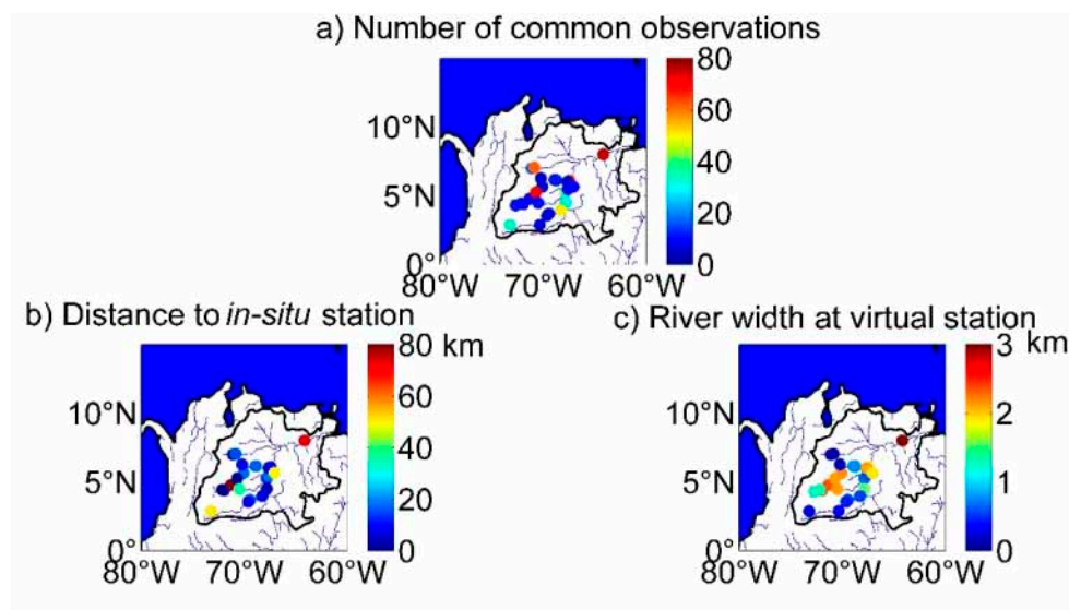
Figure 5. Comparisons between altimetry-based and in situ water levels over the Orinoco Basin. (a) Number of common observations; (b) distance between virtual and in situ stations (km); (c) river width at virtual station.
