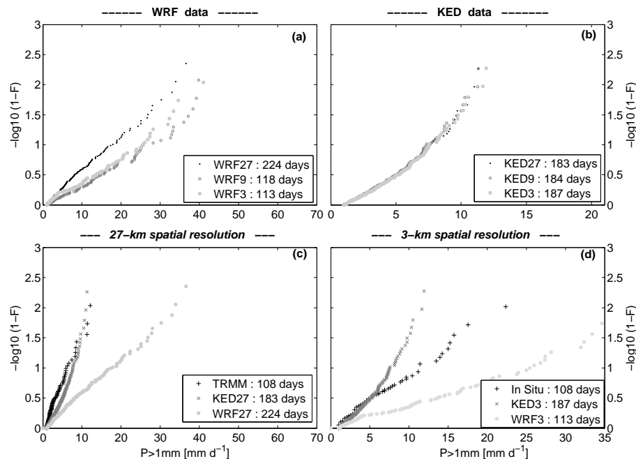
Figure 4. Frequency diagram of Corongo (station n°2) of daily precipitation data > 1 \text{ mm d}^{-1} for WRF outputs (a) and KED products (b) at three different spatial resolutions, and for all products at 27 km (c) and 3 km spatial resolution (d). Numbers in the bottom right corner indicate the number of days with precipitation > 1 \text{ mm d}^{-1} for each data set.
