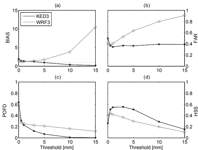
Figure 5. Daily precipitation indices: BIAS (a), false alarm rate (b), probability of false detection (c) and Heidke skill score (d). Calculated for KED3 (black) and WRF3 (gray) against rain gauge precipitation data located in the Sierra area. Scores have been evaluated for several daily precipitation thresholds: 0.1, 0.5, 1, 3, 5, 10 and 15 mm.
