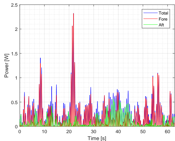
Fig. 5. Instantaneous power of the device with optimized geometric parameters and optimized PTO control parameters, for irregular waves with H_s = 4.82 cm and T_p = 1.1 s.
