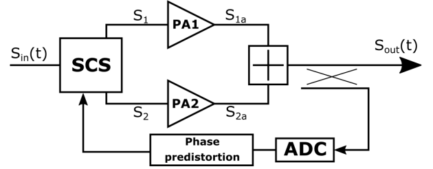
Fig. 5. Block-diagram of the proposed predistortion technique.
