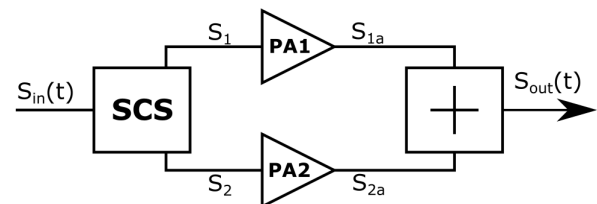
Fig. 1. Block-diagram of a LINC transmitter.
