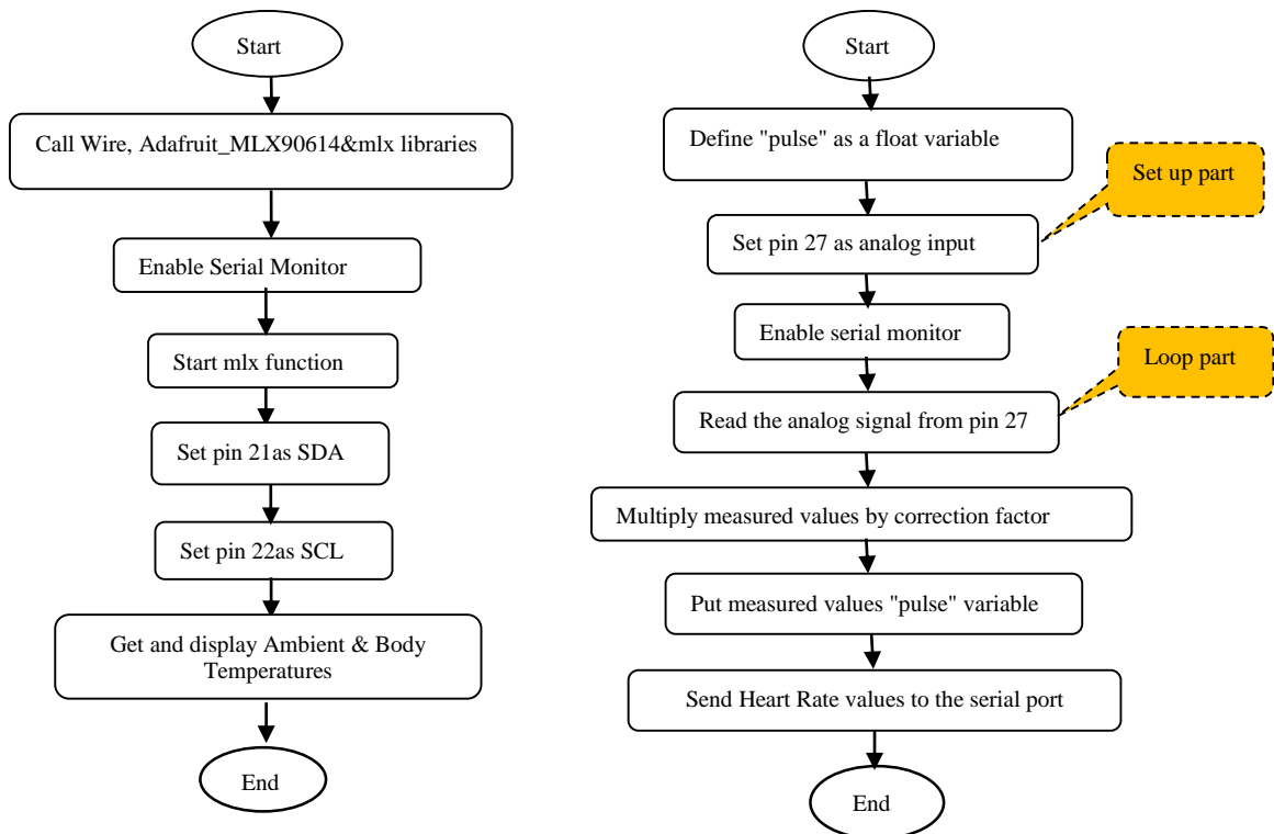
(a) Data collection process of ambient and body temperature sensor.
