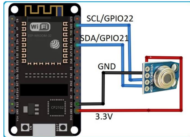
Fig. 4. Connection of the body temperature sensor with ESP32 microcontroller.
