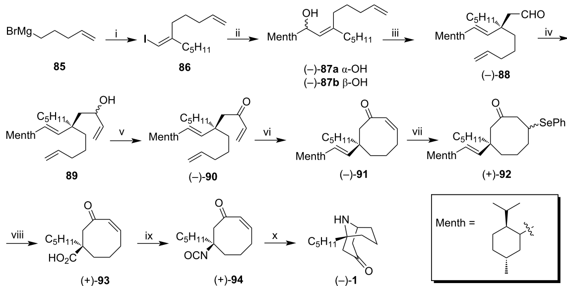
Scheme 10: Synthesis of (–)-adaline 1 . Reagents and conditions: i) 1. CuBr·DMS, Et 2 O/DMS, –42 °C; 2. 1-heptyne; 3. I 2 , THF, 82%; ii) 1. n -BuLi, Et 2 O, –78 °C to 0 °C; 2. p -menthyl-3-carboxaldehyde, 5:1 (–)- 87a / (–)- 87b , 50% (after chromatographic separation); iii) butyl vinyl ether, Hg(OAc) 2 , (10 mol %), sealed tube, 130–135 °C, 79%; iv) vinylmagnesium bromide, –78 °C; v) Dess–Martin periodinane, 83% over two steps; vi) Grubbs catalyst 2 nd gen., CH 2 Cl 2 , reflux, 74%; vii) 1. (PhSe) 2 , NaBH 4 , EtOH; 2. EtOH/THF, 99%; viii) 1. O 3 , CH 2 Cl 2 , –78 °C; 2. DMS, –78 °C to rt; 3. NaClO 2 , Na 2 HPO 4 , t -BuOH/H 2 O, 2-methyl-2-butene, 90%; ix) DPPA, Et 3 N, toluene, reflux, 65%; x) 1. CuCl, H 2 O/THF, rt to 40 °C; 2. aq K 2 CO 3 , rt, 63%.
