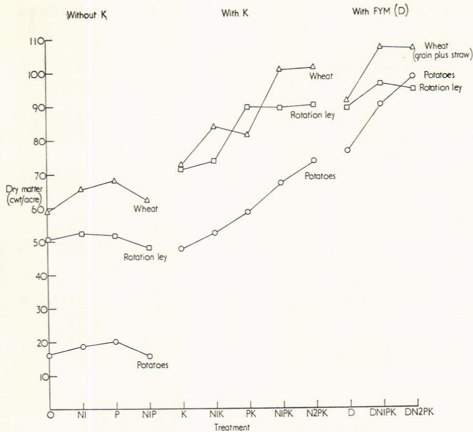
FIG. 2. The effects of N, P and K fertilisers and of FYM (D) on the yields of the three arable crops (wheat, potatoes and grass-clover ley) that responded most to K, in the Rothamsted Reference experiment, 1956-70.
