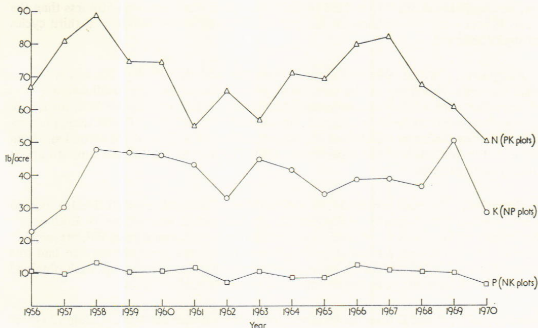
FIG. 3. The mean annual amounts (lb/acre) of N, P and K taken from the soil by the five arable crops grown on the Rothamsted Reference plots from 1956-70. Mean of five crops for P and K, mean of four (excluding ley) for N.
