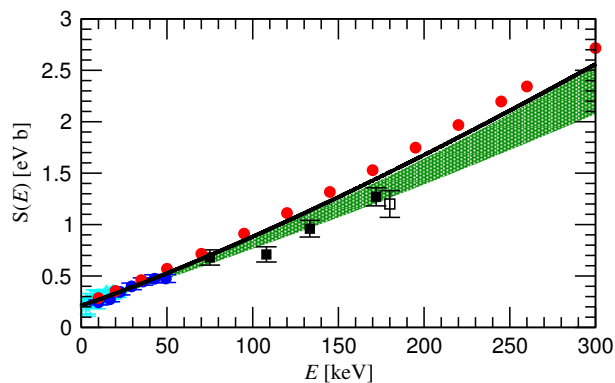
Figure 1. The astrophysical S -factor of the p+d \rightarrow {}^3\text{He} + \gamma radiative capture as function of the center of mass energy. The calculation of Ref. [3] is represented as red dots, the green band corresponds to the polynomial fit of Ref. [7], the black line reports the study of Ref. [6], while the remaining symbols are the experimental data of Refs. [8, 9, 10, 11].
