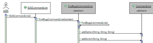
Fig. 21 FindBugs GUID2CommandLine diver output
