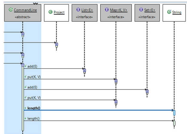
Fig. 20 FindBugs addOption diver output
