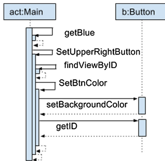
Fig. 5 Sequence diagram for an execution path in Fig. 2
