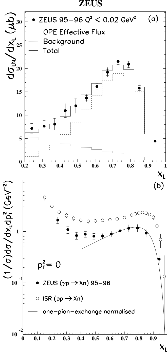
Figure 8: (a) The differential cross section for photoproduction of leading neutrons with \theta_n < 0.8 \text{ mrad} , d\sigma^{LN}/dx_L , at \langle W \rangle = 207 \text{ GeV} . The solid histogram shows the result of a fit to the data using the OPE effective flux factor, f_{\text{eff}} of Eq. (8), shown as the dashed histogram, plus a background term \propto (1 - x_L) , shown as the dotted histogram. (b) The normalised cross section for \gamma p \rightarrow Xn at p_T^2 = 0 (solid points). Also shown (open circles) are data from the ISR for pp \rightarrow Xn [28]. The curve is the expectation of the one-pion-exchange model for hadron-hadron data scaled by 0.41. In both (a) and (b), the statistical uncertainties are shown by the inner error bars and the statistical and systematic uncertainties added in quadrature by the outer bars. Points for x_L < 0.5 ( x_L > 0.5 ) are dominated by statistical (systematic) uncertainties (see Table 1).
