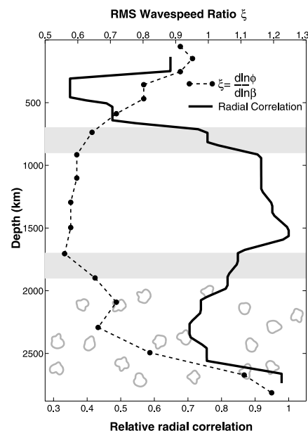
Fig. 1. Depth variation of two global diagnostics deduced from recent tomographic models (2, 32). The radial correlation (solid line) (12) is a measure of the continuity of structure in radial direction. For our purposes the absolute values are less important than the relative variations, which reveal a reduced correlation of structure between 400 and 1000 km and between 1600 and 2500 km depth. The dashed line depicts the radial variation of the root mean square (RMS) amplitude of relative variations of bulk sound and shear wavespeed, \zeta = d \ln \phi / d \ln \beta , after (32); see (30) for explanation of symbols. The open (gray) symbols mark the depth range where scattering of short-period PKP waves may occur (35).
