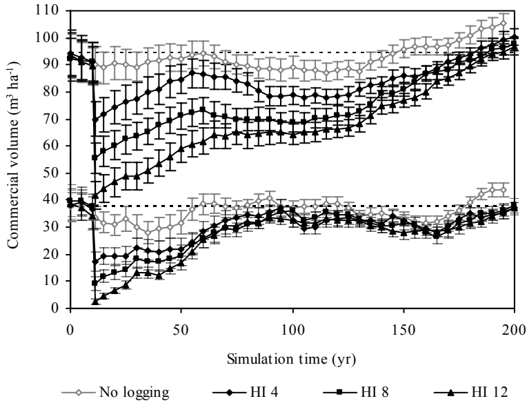
Figure 2 Mean \pm 1 SE (error bars) of standing commercial volume over simulation time for 6 scenarios with logging simulated once at year 10 and one simulation without logging. The 4 lines at the top represent commercial volumes for simulations with MFD of 35 cm and the lower 4 lines are volumes for the simulations with MFD of 60 cm. The graphs for the different HI are indicated with different markers (see legend). The volumes for the two lines of simulations without logging were based on the same simulations. The dotted lines show the initial volumes for each MFD.
