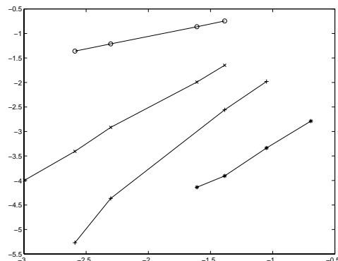
Figure 2. Plots of \log(d_\varepsilon) against \log(\varepsilon) for various resonances. The 4 : 1-resonance is plotted using 'o', the 3 : 1-resonance is using '+', the 4 : 3-resonance is using 'x' and the 6 : 1 resonance is using '*'.
