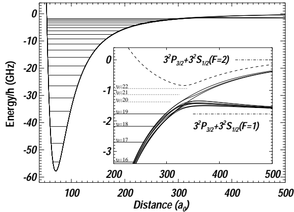
FIG. 3. Calculated potential energies and bound states for the hyperfine components of the 0_g^- . The inset shows an enlarged view for small detunings. The bound states have been indicated with the solid lines. The dotted lines indicate the positions of the hypothetical higher bound states. The dashed line indicates one of the potentials that causes the avoided crossings. Most of the 0_g^- potentials are connected to 3^2S_{1/2}(F_g=1) + 3^2P_{3/2} , only three connect to 3^2S_{1/2}(F_g=2) + 3^2P_{3/2} .
