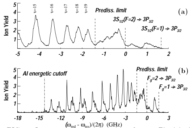
FIG. 2. Ion spectrum as a function of \omega_{red} . Fig (a) gives a more detailed view of the first 5 GHz of (b). The energy threshold for the AI process at -14.19 GHz can easily be recognized. At small detunings the vibrational series resulting from the 0_g^- displays the predicted cutoff near the predissociation limit of approximately -1.4 GHz.
