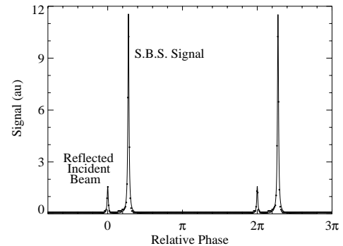
FIG. 3. Spectrum of the reflected light measured by a 1.494 GHz FSR analyzer. The solid line represents a fit through the data, including the spectrum analyzers transmission function and the frequency shift of the SBS light.
