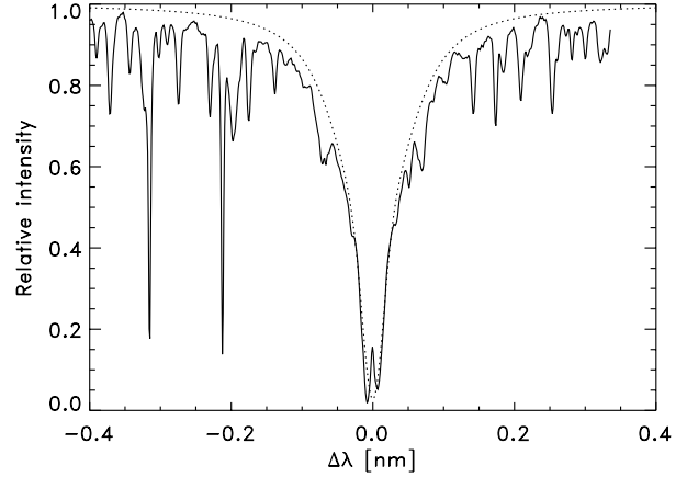
Fig. 6. The K I 769.9 nm line in a sunspot umbra. The tracing is from high-resolution FTS data obtained by O. Engvold and J.W. Brault at Kitt Peak in 1981. The dotted curve is a simple fit. It has W_\lambda = 0.107 nm
