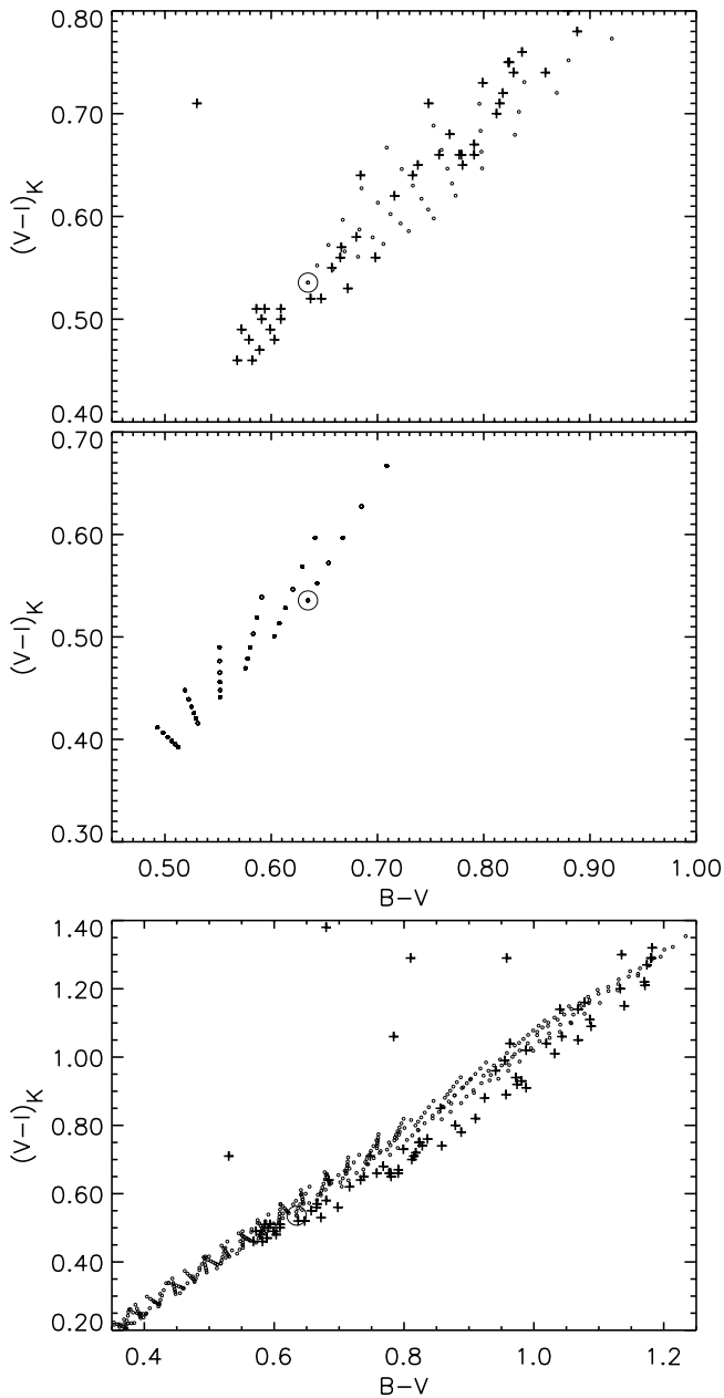
Fig. 10. Computed and observed color-color diagrams. Horizontal: dereddened B-V . The correction for interstellar reddening applied by Soderblom et al. (1993b) was \Delta(B-V) = 0.04 except for eight stars with \Delta(B-V) > 0.2 (their Table 9) of which seven make up the outlying crosses in the top and bottom panels. Vertical: Kron color (V-I)_K , without correction for interstellar reddening. Upper panel: observed values (crosses) compared with the solar spot and plage modeling. Middle panel: stellar spot and plage modeling for the solar RE model only, in order to display the computed dependencies on spots (increase to upper right) and plage (decrease to lower left). Bottom panel: observed values (crosses) compared with the stellar spot and plage modeling.
