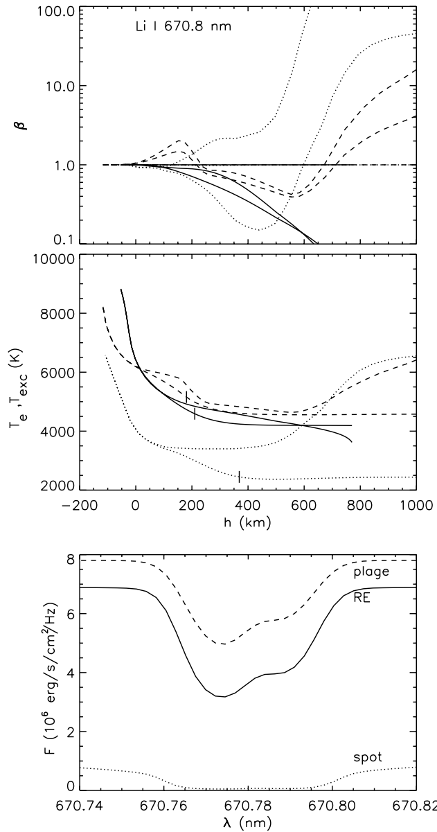
Fig. 3. Formation of the Li I 670.8 nm resonance doublet for the three solar models. Curve coding as in Fig. 2. Top panel: NLTE departure coefficients \beta = n_i/n_i^{\text{LTE}} for the 2s Li I ground state (upper curve for each pair) and the 2p upper levels of Li I 670.8 nm (lower curves). Middle panel: model temperatures T_e as in Fig. 2 (upper curve of each pair) plus line source functions in the form of excitation temperatures T_{\text{exc}} . The ticks mark locations with total optical depth unity at line center. Bottom panel: emergent flux profiles
