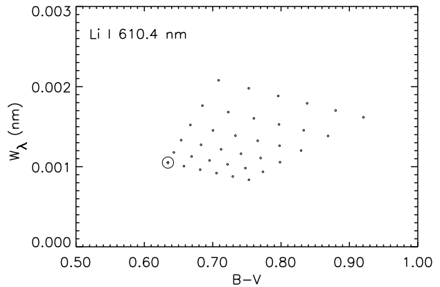
Fig. 11. Computed equivalent widths of the Li I 610.4 nm 3d-2p subordinate transition, for solar modeling as in Fig. 7
