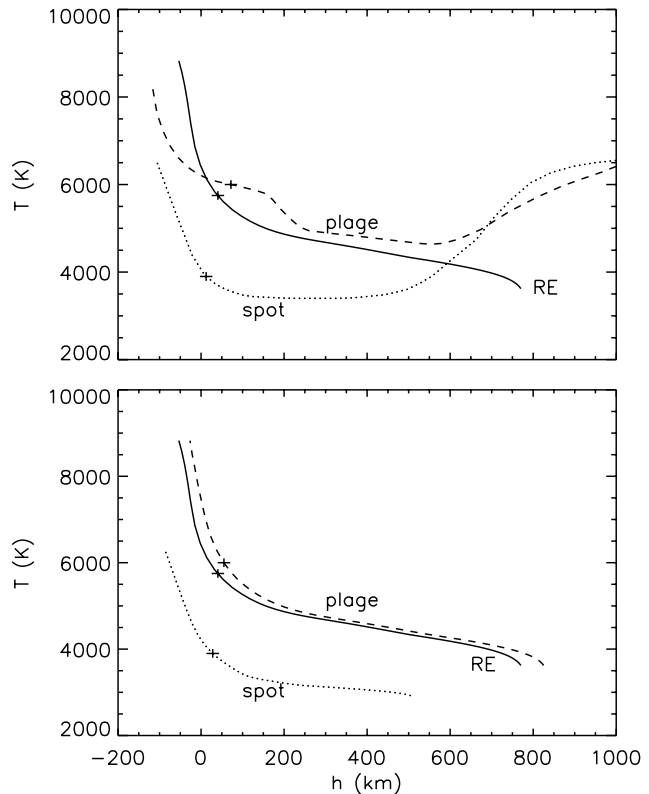
Fig. 2. Temperature stratifications. Each model is shown on its own height scale, with h = 0 km at \tau_{500} = 1 . The crosses mark the effective temperature per model. Upper panel: solar models. The radiative-equilibrium stratification (RE) is the T_{\text{eff}} = 5750 model from the Uppsala grid. The sunspot umbra and plage fluxtube stratifications are empirical models from the literature. Lower panel: stellar modeling for T_{\text{eff}} = 5750 K. The RE model is the same as in the upper panel. The spot umbra is described by an Uppsala RE model with lower (65%) effective temperature. The stratification of the plage fluxtube is derived from the RE model by requiring thin-tube magnetostatic equilibrium with the same temperature within and outside the fluxtube
