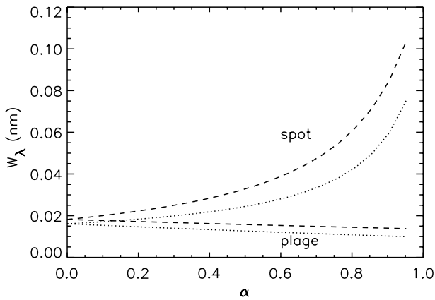
Fig. 5. Computed equivalent widths of Li I 670.8 nm (dotted) and K I 769.9 nm (dashed) against filling factor \alpha when combining the T_{\text{eff}} = 5750 RE model with sunspot umbrae and solar facular fluxtubes, respectively. The Li I and K I resonance features have similar sensitivity to magnetic activity
