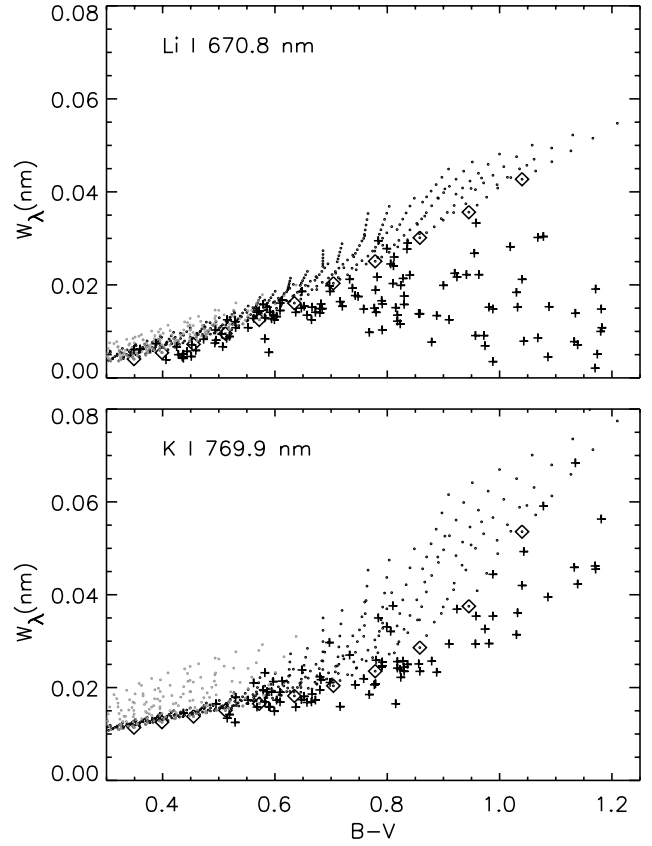
Fig. 8. Computed and observed equivalent widths of Li I 670.8 nm ( upper panel ) and K I 769.9 nm ( lower panel ) against color B-V , as in Fig. 7 but for the stellar modeling. Diamond symbols : line strength computed from the RE atmospheres. Dots : line strengths computed from mixtures of the RE atmospheres with starspots and stellar plage modeled by the simple recipes described in Sect. 2. The spot and plage filling factors \alpha_s and \alpha_p again vary each as \alpha = 0, 0.1, \dots, 0.5 . Starspots cause reddening plus line strength increase similarly to the sunspots in Fig. 7, but the stellar plage models produce opposite behavior by combining slight line strength decrease with appreciable decrease of B-V . Crosses : observations by Soderblom et al. (1993a), the same as in Fig. 1
