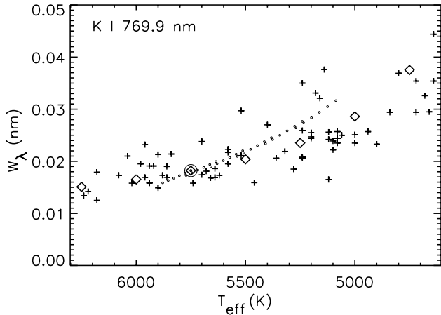
Fig. 9. Computed and observed equivalent widths of KI 769.9 nm as in Fig. 7, but plotted against effective temperature T_{\text{eff}} rather than color B-V . The crosses mark the observations of Soderblom et al. (1993a) at the T_{\text{eff}} values tabulated in their paper. The latter are based on standard B-V to T_{\text{eff}} conversion, whereas we have evaluated T_{\text{eff}} explicitly per atmospheric model combination (dots). The sunspot and solar plage fluxtube filling factors \alpha_s and \alpha_p again vary each as \alpha = 0, 0.1, \dots, 0.5 , but all dots happen to fall on a single curve which is rather close to the locus of the RE predictions (diamonds)
