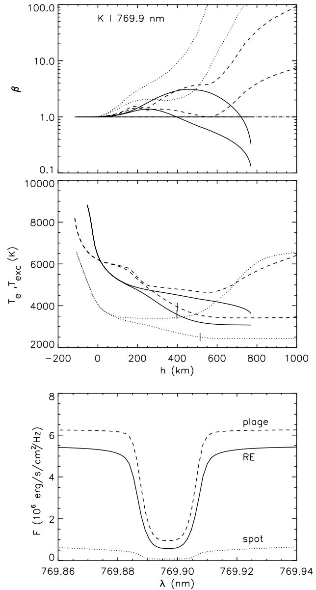
Fig. 4. Formation of the K I 769.9 nm resonance line for the three solar models. Panel layout and curve coding as in Fig. 3. The departure coefficients in the upper panel are for the 4s K I ground state (upper curve of each pair) and the 4p upper level of K I 769.9 nm
