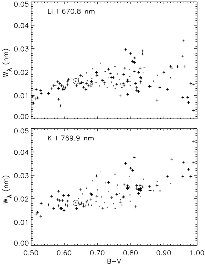
Fig. 7. Computed and observed equivalent widths of Li I 670.8 nm ( upper panel ) and K I 769.9 nm ( lower panel ) against color B-V , for the solar models. Sun symbol : line strength computed from the T_{\text{eff}} = 5750 RE model. Dots : line strengths computed from mixtures of solar RE, sunspot and solar plage models. The spot and plage filling factors \alpha_s and \alpha_p vary each as \alpha = 0, 0.1, \dots, 0.5 . The dots mark all combinations, with the rightmost dot giving the result for a solar-type (but rather non-solar-like!) star that is covered half by sunspot umbrae and half by facular fluxtubes. Sunspots cause reddening plus increase of Li I and K I equivalent width. Solar plage causes yet larger reddening plus slight decrease of Li I and K I equivalent width. Crosses : observations by Soderblom et al. (1993a), the same as in Fig. 1
