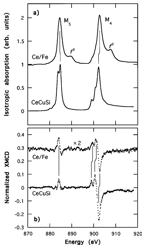
FIG. 1. Isotropic (upper panel) and XMCD (lower panel) spectra obtained for a Ce(10 Å)/Fe(30 Å) multilayer and CeCuSi [4] at the Ce- M_{4,5} absorption edges. The intensity of the M_5 edge isotropic spectra of the two samples has been arbitrarily set to unity. The XMCD spectra have been normalized to 100% circular polarization rate.
