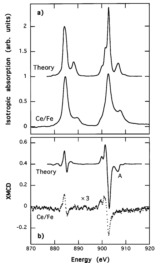
FIG. 3. Comparison between the experimental data of the Ce/Fe multilayer and the results of the model described in the text. Top panel, Ce- M_{4,5} isotropic spectra; lower panel, XMCD spectra. The intensity of the two M_5 edge isotropic spectra has been set to unity. The origin of the energy axis has been chosen in order to align the positive peaks at correspondence with the M_5 edge of the theoretical and experimental XMCD spectra.
