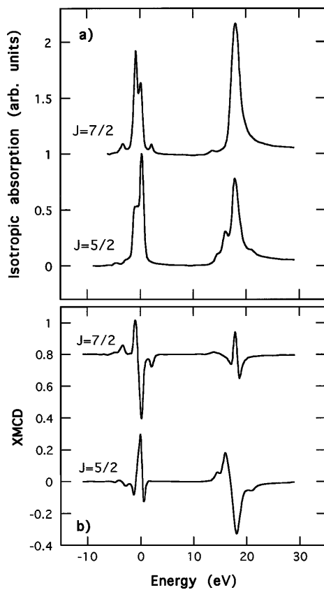
FIG. 2. Ce- M_{4,5} isotropic (top panel) and XMCD (lower panel) spectra obtained for the J = \frac{5}{2} and J = \frac{7}{2} states calculated for the ion \text{Ce}^{3+} . The zero of the energy axis has been chosen at correspondence with the maximum in the M_5 edge of the J = \frac{5}{2} XMCD spectrum. The intensity of the M_5 edge of the J = \frac{5}{2} isotropic spectrum has been set to unity.
