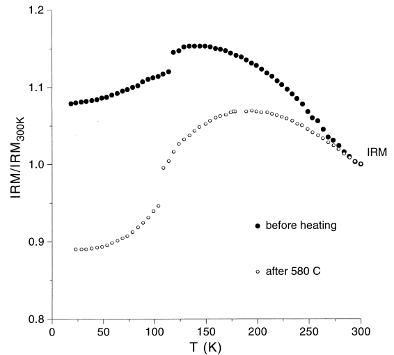
Fig. 8. Low-temperature measurements. The IRM was imparted with a 2.5-T field at 300 K (27°C), before cooling the specimen to 20 K (−253°C) in a zero field.
