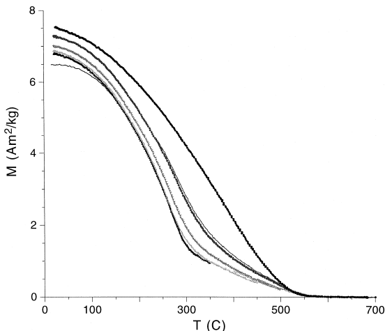
Fig. 7. A typical example of successive thermomagnetic M_s - T runs up to 350, 450, 500, 580 and 700°C. Lines (dotted lines) denote heating (cooling) curves.
