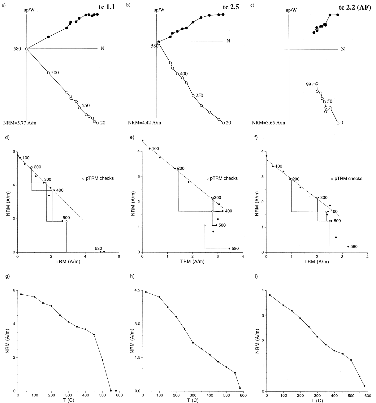
Fig. 1. (a) NRM thermal demagnetization diagram (Zijderveld, 1967) for samples 1.1 and 2.5. (c) AF demagnetization diagram for sample 2.2; another specimen from this paleomagnetic core was used for Thellier–Thellier paleointensity experiments. (d,e,f) NRM versus TRM intensity and (g,h,i) NRM thermal decay curves for samples 1.1, 2.5 and 2.2.
