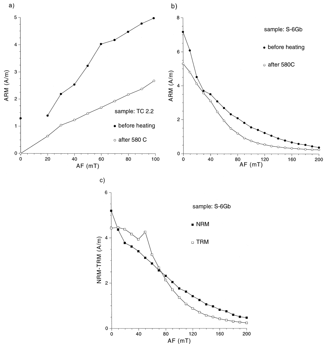
Fig. 3. (a) ARM acquisition curves. (b) ARM (closed circles before heating; open circles after heating) and (c) NRM (closed squares), TRM (open squares) versus AF demagnetization. Results shown in (b) and (c) are from the paleointensity determinations on sample S-6Gb by Gonzalez et al. (1997).
