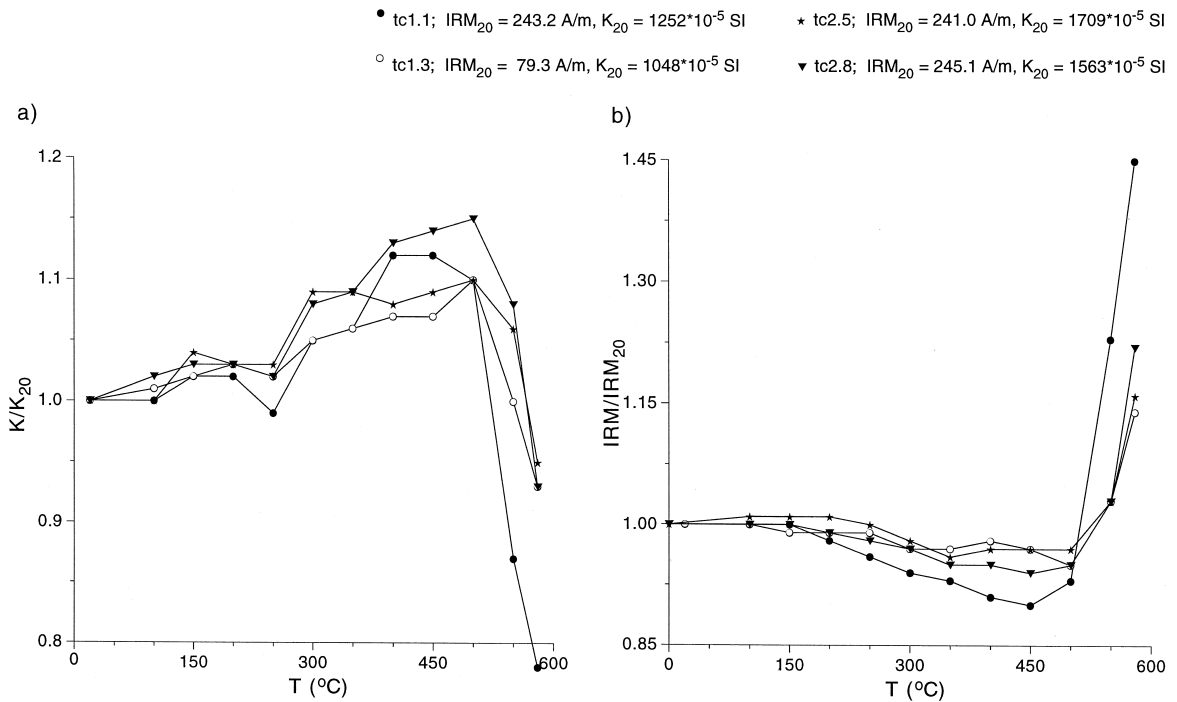
Fig. 2. (a) K and (b) IRM after heating. Both parameters are measured at room temperature and normalized on K and IRM values before heating. K and IRM values before heating are shown in the right column.
