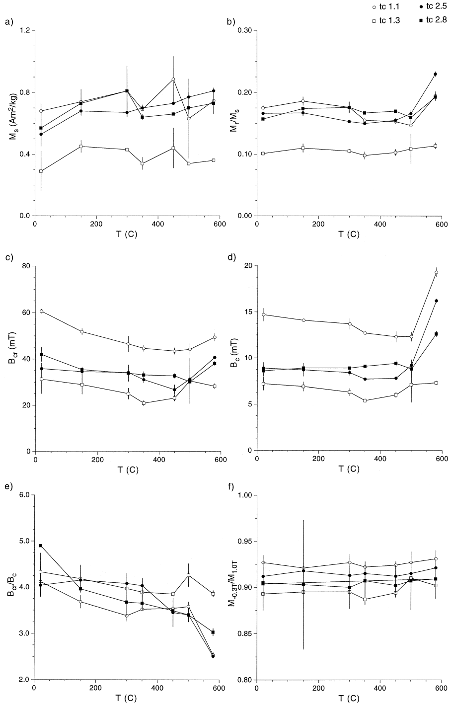
Fig. 6. Changes in (a) M_s , (b) M_r/M_s , (c) B_{cr} , (d) B_c , (e) B_{cr}/B_c and (f) S ( = M_{-0.3T}/M_{1.0T} ) ratios after heating. Sample TC 1.3 shows the weakest variations in hysteresis parameters during heating. This sample also has the lowest coercivities and remanence ratios and smallest variations in K and IRM (Fig. 2).
