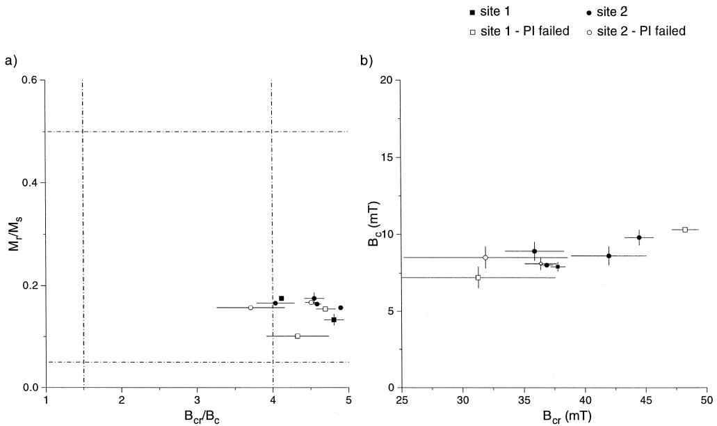
Fig. 5. Hysteresis parameters [(a) M_r/M_s , versus B_{cr}/B_c (b) B_c versus B_{cr} ] at room temperature. Open (closed) symbols denote samples, which Thellier–Thellier paleointensity experiments failed (passed).
