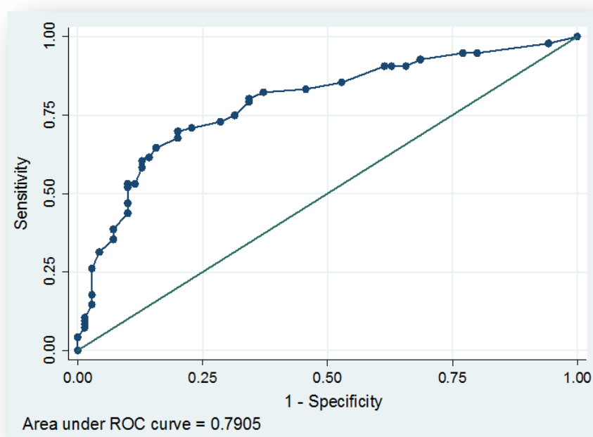
Figure 11: ROC curve analysis of main multivariate logistic regression model
