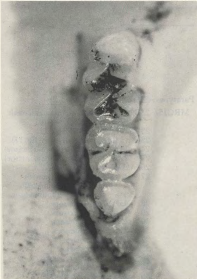
Figure 17 Proodontomys cookei n. sp. Left maxilla MRCIS/23D showing occlusal aspect of toothrow. x 14,5.
