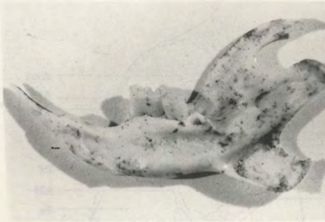
Figure 16 Holotype right mandible MRCIS/23A of Proodontomys cookei n. sp., internal aspect. Intact except for loss of third molar. x 5. (For external aspect, see fig. 14).
