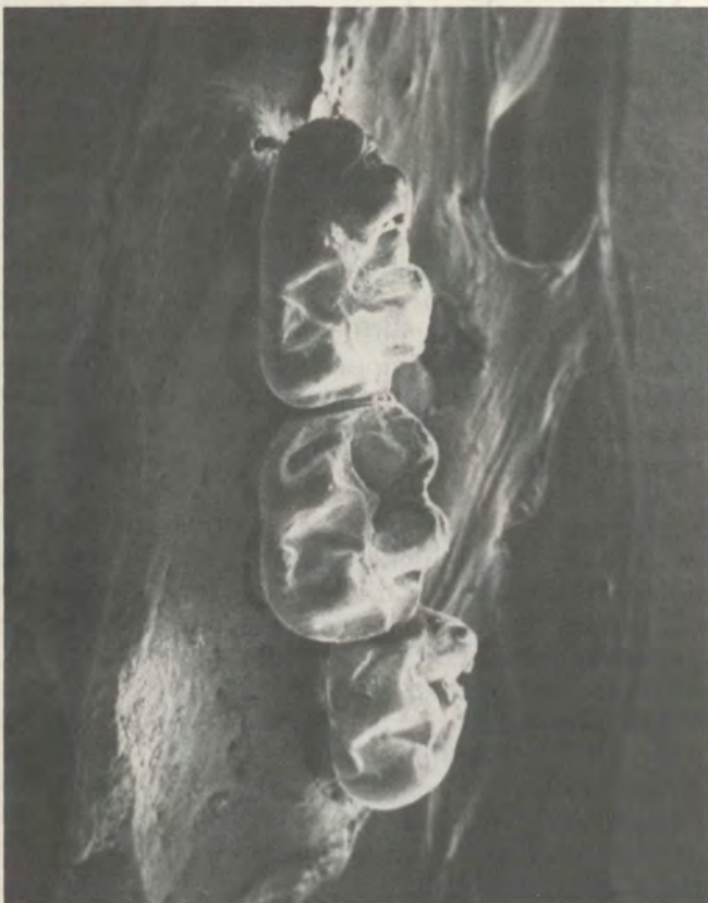
Figure. 19 Stenodontomys darti . Left lower toothrow, SEM photograph x 20. Third molar about 2/3 size of 2nd, not as reduced as in Mystromys , Mus and especially the Dendromuridae; axis of M 3 markedly offset from that of M 2 as in many cricetines but not Mystromys .
