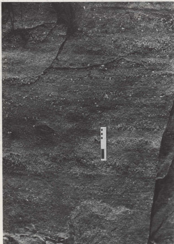
Fig. 11 Internal structure of longitudinal bar showing systematic variation in grain size, and depositional couplets of gravel-rich and gravel-poor very coarse sandstone.
