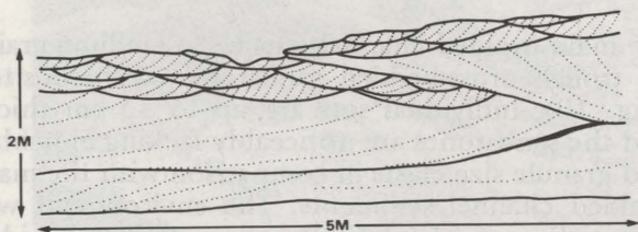
Fig. 9 Stratification sequence in braided channel-fill sandstone. Trough cross-bedding (sinuous crested dunes) dominates and shows an abrupt upward decrease in scale. A foreset cross-bedded unit of transverse bar origin occurs at the bottom left. Drawn from a photograph.
