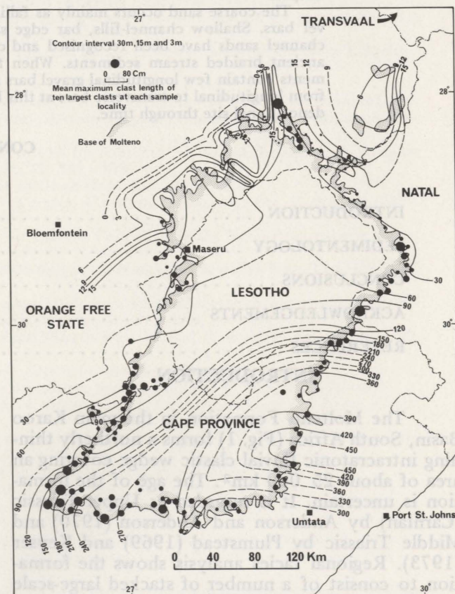
Fig. 2 Clast size and isopach map of total thickness of the Moltano Formation. Note the local increase in clast size and thickness along the northern margin of the outcrop, contrary to regional trends. The dome-shaped feature delineated by the isopach contours in the northeast is known as the Harrismith dome (Turner, 1975).
