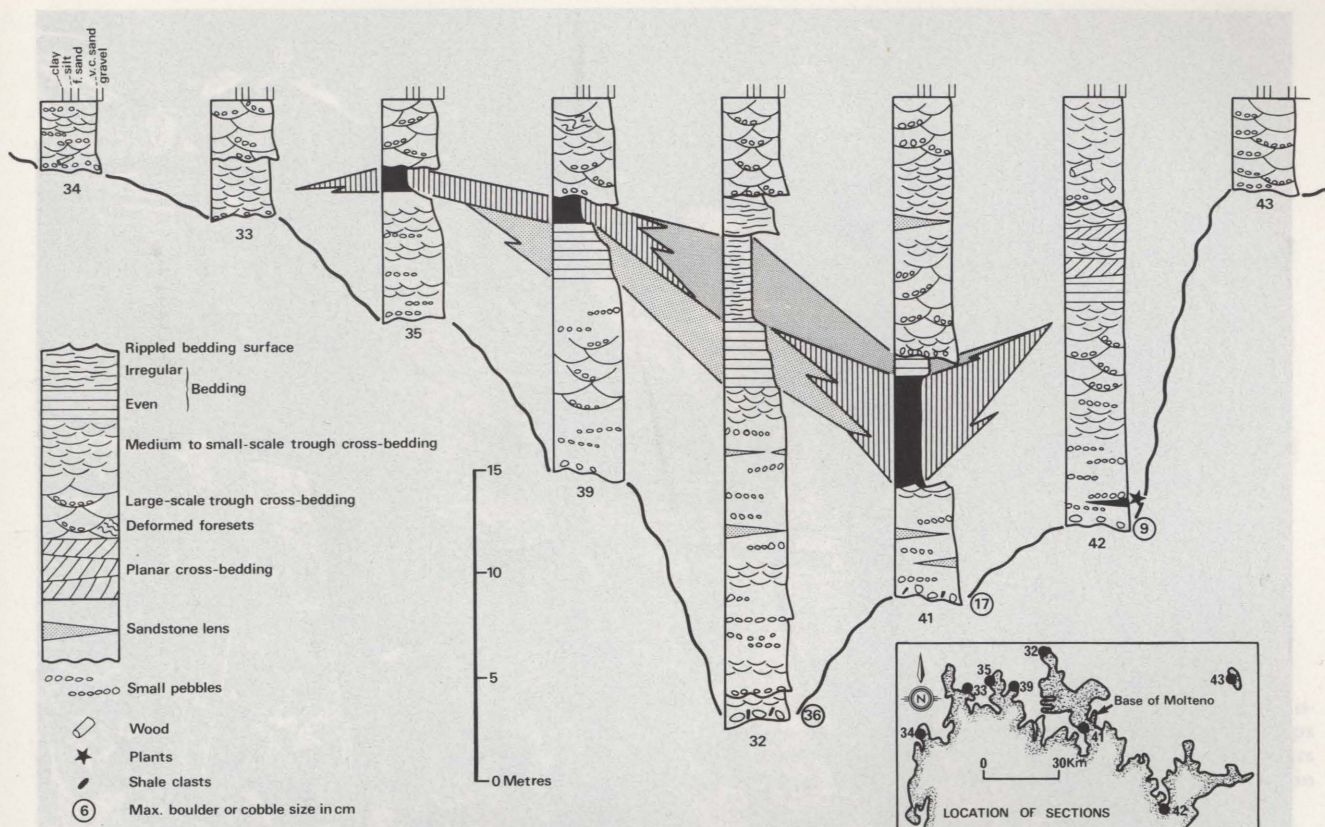
Fig. 10 Correlation of sections along the northern margin of the Molteno Basin showing lateral variations in thickness and stratification.
