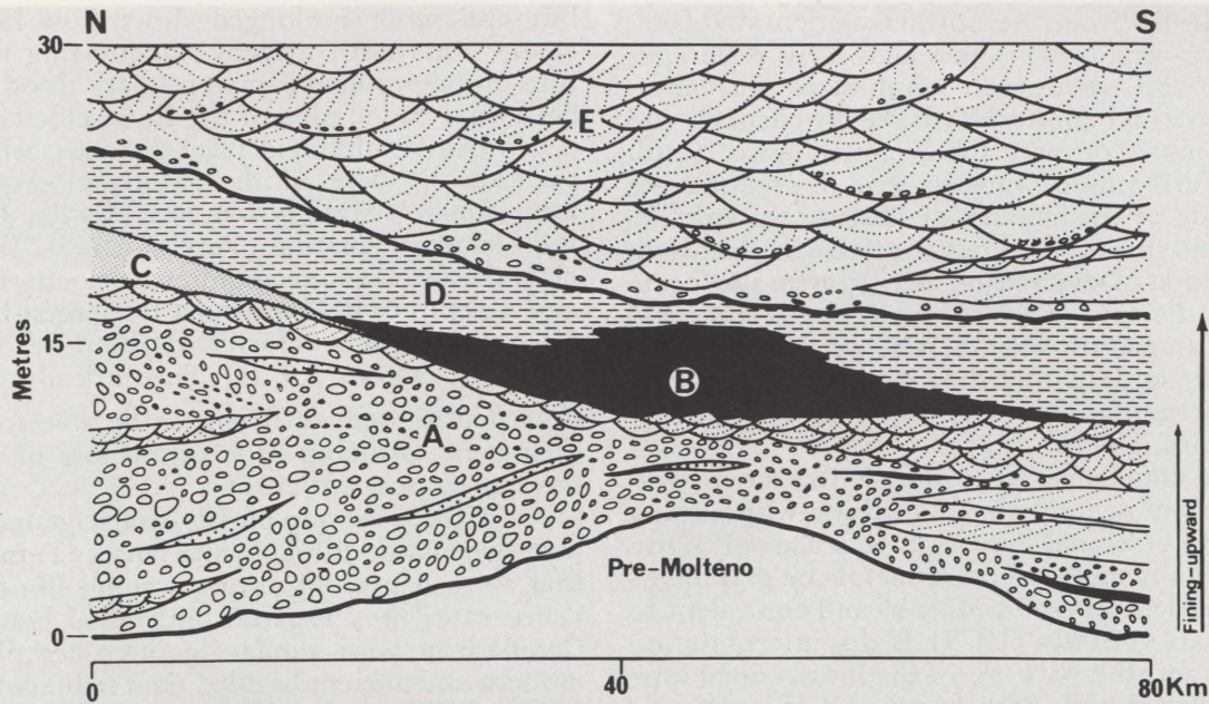
Fig. 3 Generalised section showing characteristic features of the Molteno Formation along the north-central margin of the basin. General transport direction from south to north. (A) The lower part of the formation (Indwe Sandstone Member) consists of pebble and granule conglomerate (gravel) overlain by trough cross-bedded very coarse, pebble and granule rich sandstone. The conglomerate is thicker and generally coarser in the north (distal) becoming thinner and slightly finer to the south (proximal) accompanied by a change in the dominant stratification type from longitudinal gravel bars to more sandy transverse bars and subordinate gravel bars confined to a thin basal zone. The remainder of the succession consists of (B) shale, (C) fine-medium sandstone, (D) silty-shale and (E) coarse granule and pebble rich trough cross-bedded sandstone. The section line extends from Danielsrust to Oliviershoek Pass and corresponds to sections 32, 41 and 42 in Fig. 10.
