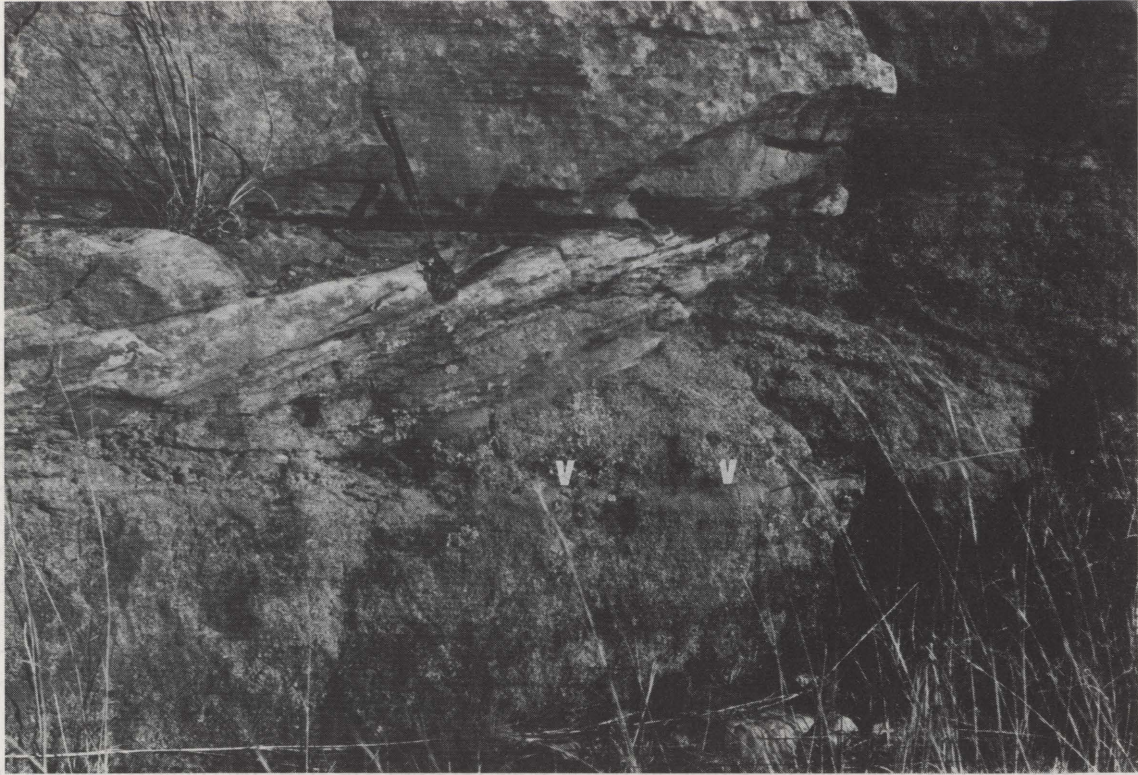
Fig. 7 Bar edge sand wedge with low angle foresets. A thin bar top sand occurs below the wedge (arrowed) which is overlain by a thicker, erosively based sandstone representing part of a sand-filled channel cut into the gravel bar top. General transport direction towards observer.
