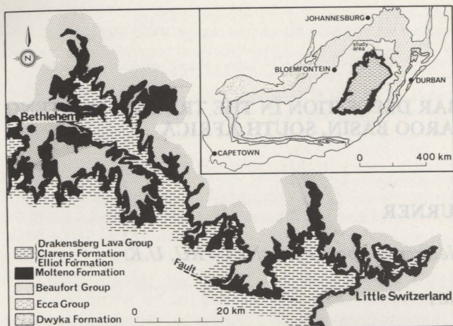
Fig. 1 Generalised stratigraphic and locality map of the study area. The inset map shows the Karoo Basin with study area enclosed.
