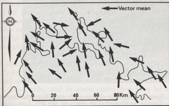
Fig. 4 Palaeocurrent map of the northern distal margin of the Molteno Basin. Vector means based on 1018 measurements of the axes of trough cross-bedded sets.
