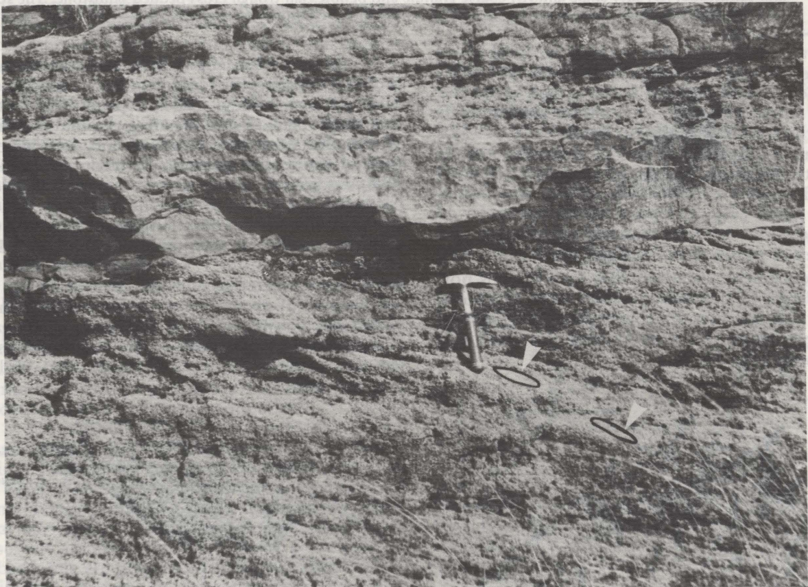
Fig. 6 Thin channel-fill sandstone within gravel bar sequence. Note the presence of low angle stratification dipping into the channel on the right, and small pock marks indicating weathered shale clasts on the left. Low angle gravel bar foresets dipping to the right can be seen beneath the channel-fill sandstone. Some foresets contain small, discoidal sandstone intraclasts (outlined in black and arrowed in white) with their long axes preferentially aligned down the foreset slope. General transport direction towards the observer.
