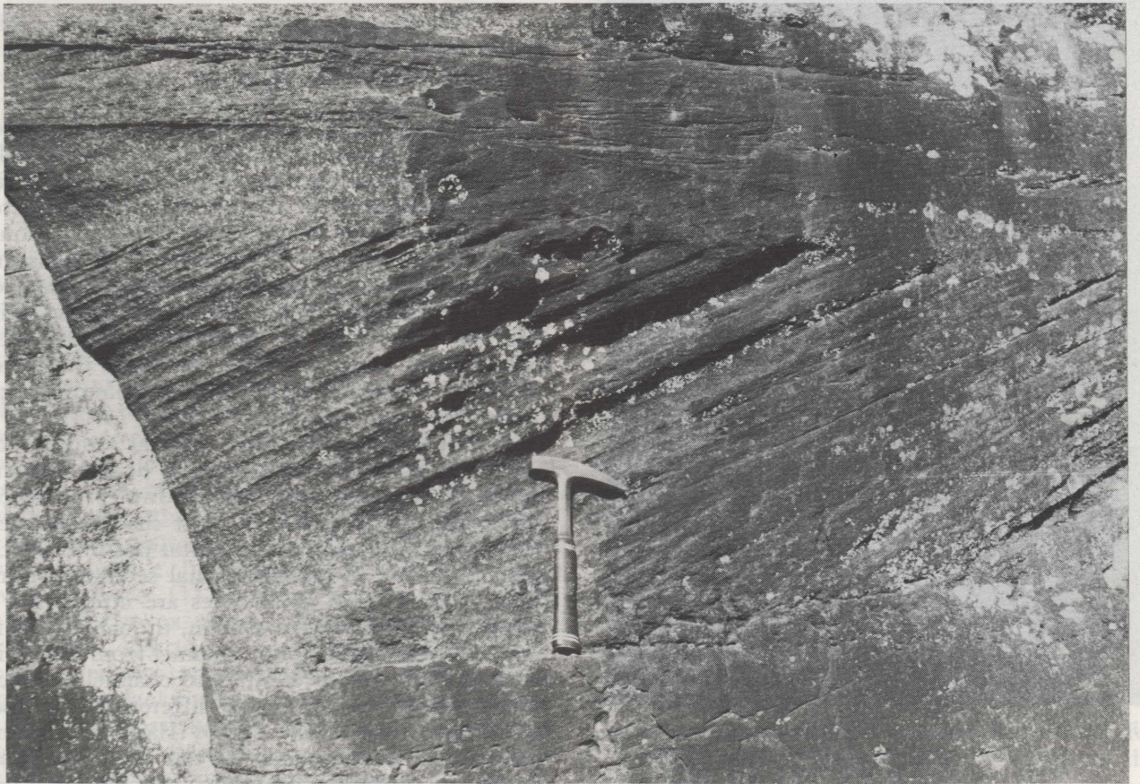
Fig. 13 High angle simple planar set of transverse bar origin overlain by a separate sedimentation unit of small trough cross-lamination. Note the curvature of the bar surface and its tapering-off towards the bar tail to the right.
