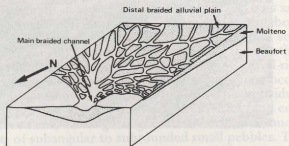
Fig. 5 Generalised depositional model for the Molteno Formation along the north-central distal margin of the basin.
