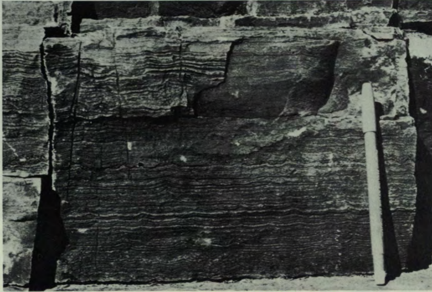
Fig. 6. Low amplitude stromatolitic bedding on elongate mounds. (Scale : 15 cm in length)
