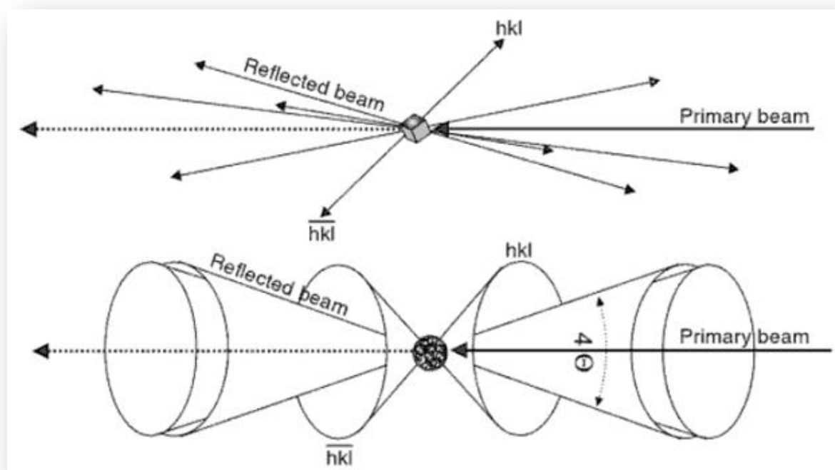
Figure 1.15. Comparison between diffraction from A – a single crystal and B – a randomly orientated powder sample with Debye-Scherrer cones 39
