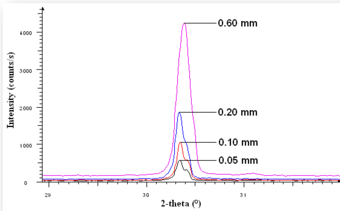
Figure 2.4. The variation in intensity of the LaB 6 1 1 0 peak as a function of (FDS) size
