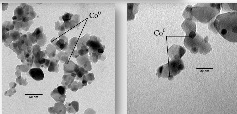
Figure 3.128. TEM images of the Co/Degussa P25 catalyst after reduction
