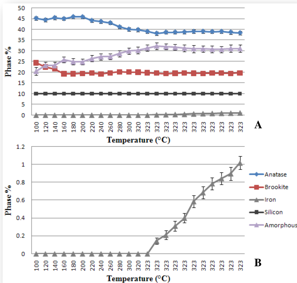
Figure 3.121. Quantitative phase analysis of the Fe/NSA catalyst during reduction with 100% H 2 : A – all phases and B – iron (average GoF of 1.13)
