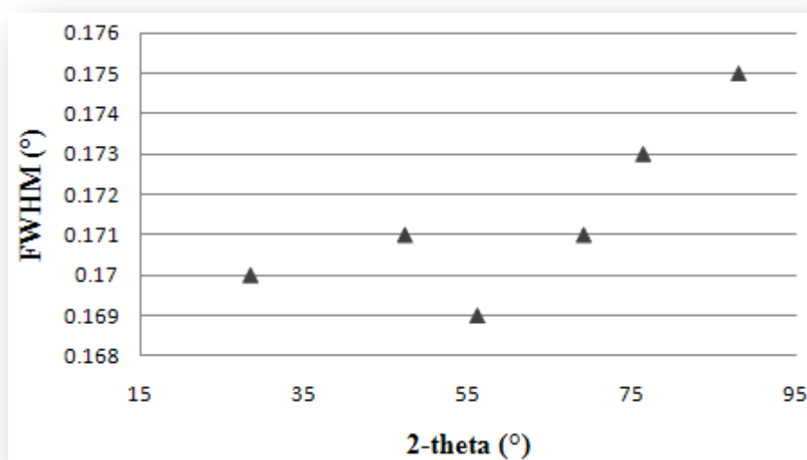
Figure 2.7. The variation of the FWHM of the NIST Si (SRM640c) diffraction peaks, collected on the WITS D8, with increasing 2-theta
