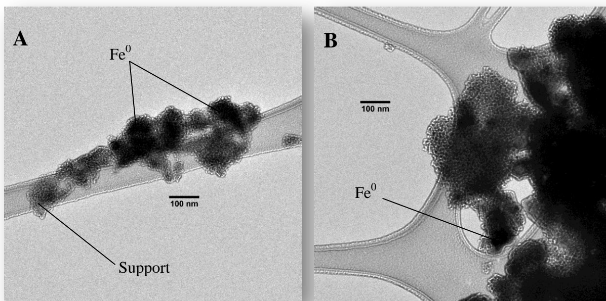
Figure 3.123. TEM images of the Fe/NSA support after reduction: A – small iron-support cluster and B – sample representation
