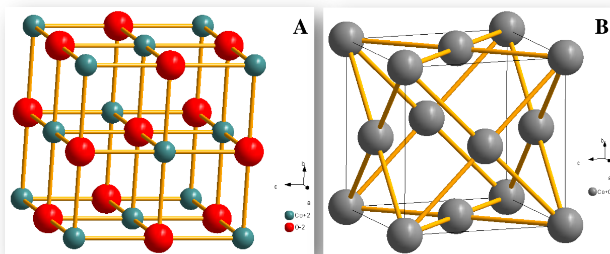
Figure 3.125. Crystallographic representations of A - \text{CoO} (cubic Fm\bar{3}m ) 73 and B – metallic cobalt (cubic Fm\bar{3}m ) 74
