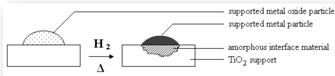
Figure 3.150. Formation of the amorphous interfacial material between metal particles and TiO_2 supports during reduction
