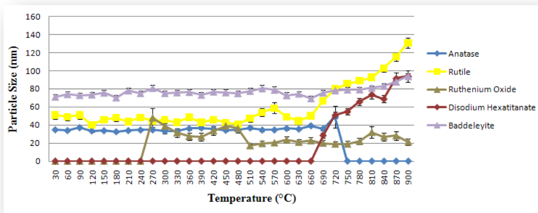
Figure 3.80. Particle size changes of the constituent phases during the heat treatment of the Ru/Degussa P25 catalyst
