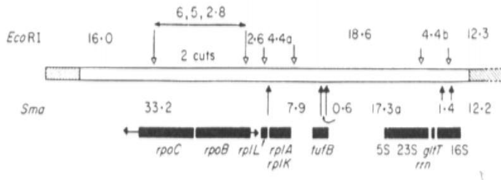
Figure 6. Genetic map of a portion of the \lambda rif^d 18 chromosome. Selected restriction endonuclease recognition sites are indicated with arrows. Distances between these are in %- \lambda units (from Lindahl et al. , 1977).
