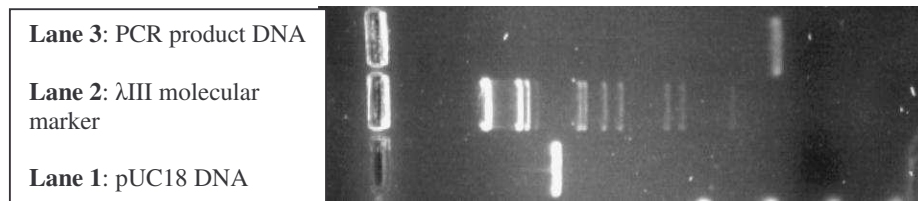
Figure 15. 1.0% agarose gel showing extracted PCR product and pUC18 DNA after Bam HI and Hind III double digestions.
