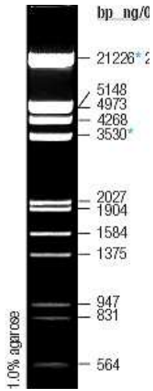
\lambda III molecular marker
