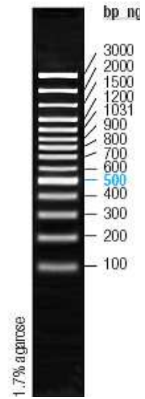
GeneRuler 100bp DNA ladder
