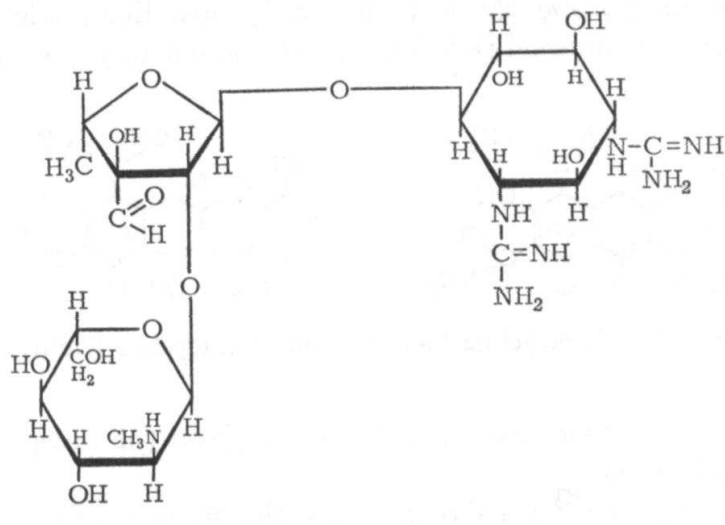
Figure 4. Molecular structure of streptomycin (from Spirin and Gavrilo, 1969).
