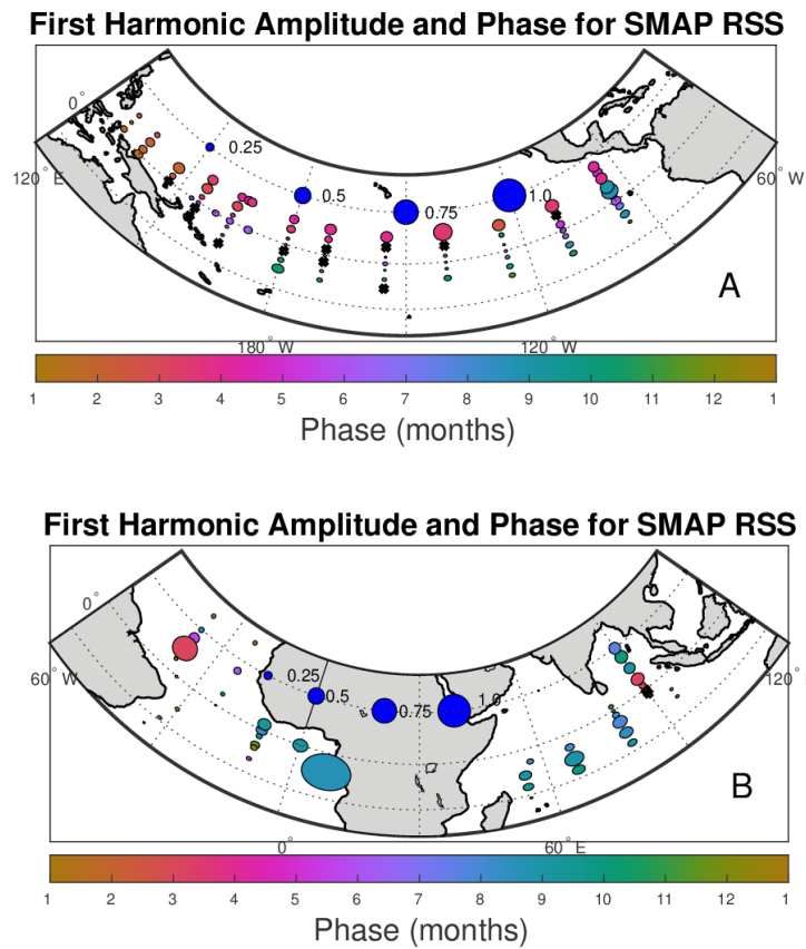
Figure 5. As in Figure 3, but for the SMAP RSS data. (A) Pacific basin. (B) Atlantic and Indian basins.
