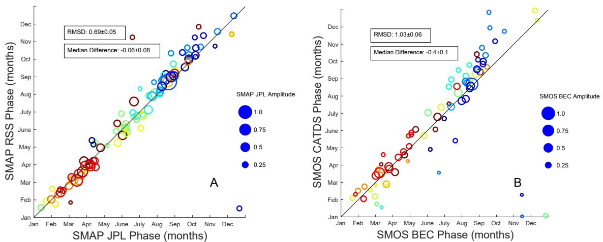
Figure 8. As in Figure 7. Comparisons are (A) SMAP RSS vs. SMAP JPL and (B) SMOS CATDS vs. SMOS BEC.
