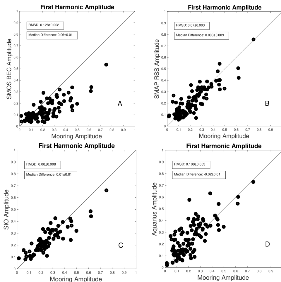
Figure 9. Scatterplots of first harmonic amplitude vs. mooring amplitude. A light black line shows a one-to-one correspondence. Boxes in each panel show RMSD and median difference (mooring-comparison). Comparison amplitudes are (A) SMOS BEC, (B) SMAP RSS, (C) SIO, (D) Aquarius. For completeness, all first harmonic amplitude comparisons are shown in the supplemental materials (Table S3).
