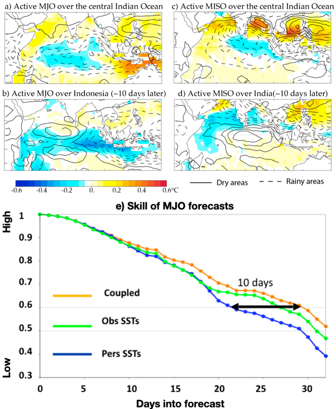
Fig. 4. Atmospheric convection perturbation (outgoing longwave radiation, contours every 10 W m -2 ) and sea surface temperature (SST; colors) composites of two successive phases of (a),(b) the Madden–Julian oscillation (MJO) during December–March and (c),(d) the monsoon intraseasonal oscillation (MISO) during June–September. (e) MJO forecast skill as a function of lead time (days) for forecasts with fixed SST, observed SST, and active ocean–atmosphere coupling. The MJO and MISO modulate tropical rainfall during boreal winter and summer, respectively. They are associated with SST and oceanic mixed layer processes, which need to be better observed to improve their forecasts.
