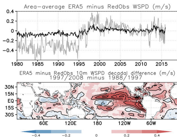
FIG. 6. (a) Time series of area-averaged ERA5 minus RedObs 10-m wind speed ( \text{m s}^{-1} ) over the global oceans (black) and eastern tropical Pacific (180°–290°E, 20°N/S domain) (gray). (b) Decadal difference (1997–2008 minus 1988–97) of ERA5 minus RedObs 10-m wind speed ( \text{m s}^{-1} ).
