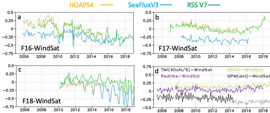
FIG. 5. Globally averaged (60°N/S) SSMIS (a) F16 , (b) F17 , and (c) F18 minus WindSat 10-m wind speeds ( \text{m s}^{-1} ) for three different retrieval algorithms. WindSat data are RSS retrievals. Differences are made with total signal, not anomalies. (d) 10-m wind speed differences of individual sensors and ensemble RedObs with WindSat. ASCAT wind speeds are RSS V7 products and TMI and GPM winds are produced by the SeaFlux v3 retrieval algorithm (Roberts et al. 2020). A 3-month running smoother has been applied to each time series.
