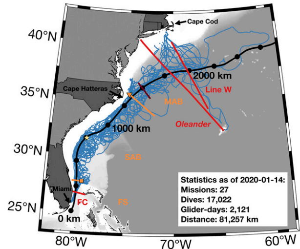
FIG. 1. Trajectories of Spray glider missions in the Gulf Stream (blue). Locations of sustained in situ Gulf Stream observations from other programs (red): the Florida Cable (FC) a part of the Western Boundary Time Series; the Oleander line; and Line W. The mean 40-cm SSH contour averaged over 16 calendar years (1 Jan 2004–31 Dec 2019) represents the mean Gulf Stream position and provides an along-stream coordinate system (black with dots every 250 km). Orange lines delineate different dynamical regions: the Florida Strait (FS), South Atlantic Bight (SAB), and Middle Atlantic Bight (MAB). The orange triangle indicates the location of “The Point” near Cape Hatteras, and the orange square shows the northwesternmost point of Little Bahama Bank at the 500-m isobath. The yellow star denotes the location of the Charleston Bump. The PEGASUS line near 73°W is shown in maroon. From south to north, Florida, North Carolina, and the New England states are highlighted in dark gray, and important locations are indicated with arrows. Glider mission statistics are displayed in the lower right.
