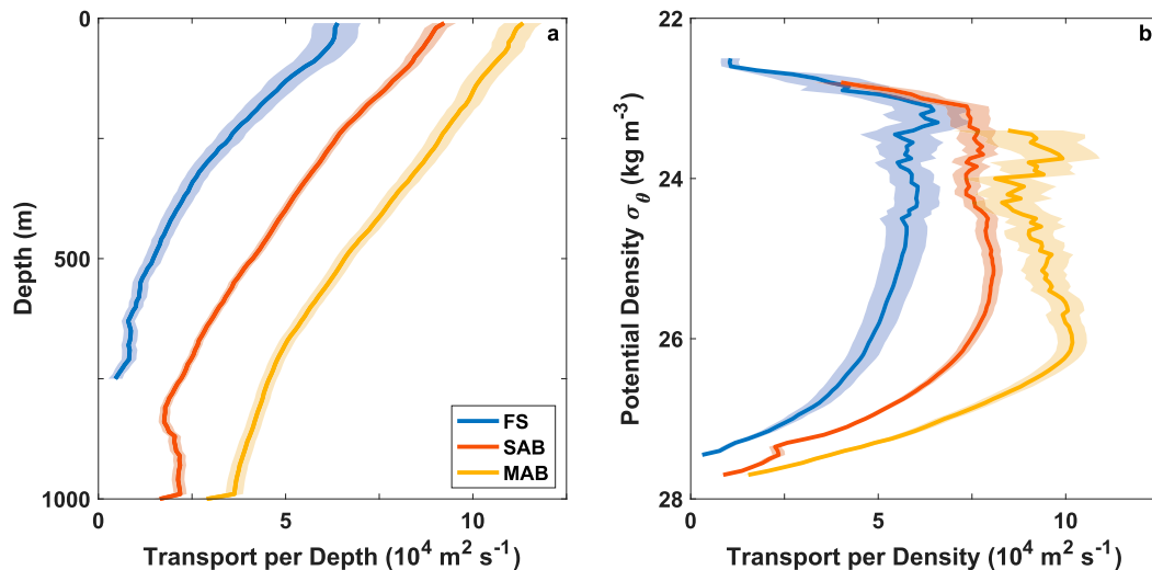
FIG. 11. Vertical structure of volume transport in the FS, MAB, and SAB as a function of (a) depth and (b) potential density \sigma_\theta . The shading indicates the respective standard error of the mean.
