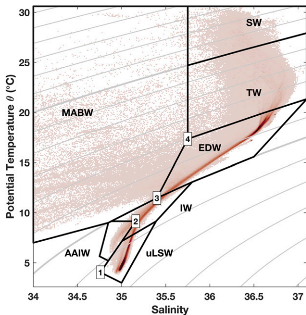
FIG. 13. Joint probability density function for potential temperature \theta and salinity using all available glider observations. Gray contours are isopycnals with a contour interval of 0.5 \text{ kg m}^{-3} and the 24.0 and 27.0 \text{ kg m}^{-3} isopycnals bold. Black regions delineate the following water classes: Gulf Stream surface water (SW), Gulf Stream thermocline waters (TW), Eighteen Degree Water and related subthermocline waters (EDW), upper Labrador Sea Water (uLSW), Antarctic Intermediate Water (AAIW), other intermediate waters (IW), and fresher waters that have been influenced by the Middle Atlantic Bight shelf waters (MABW). The MABW region extends to much lower salinities than shown to capture the freshest waters encountered. Coordinates of the numbered vertices used to delineate water classes are given in Table 2. Water class boundaries not including numbered vertices either follow isolines of potential density \sigma_\theta , potential temperature \theta , or salinity, or they are arbitrarily positioned outside of the range of observed water properties.
