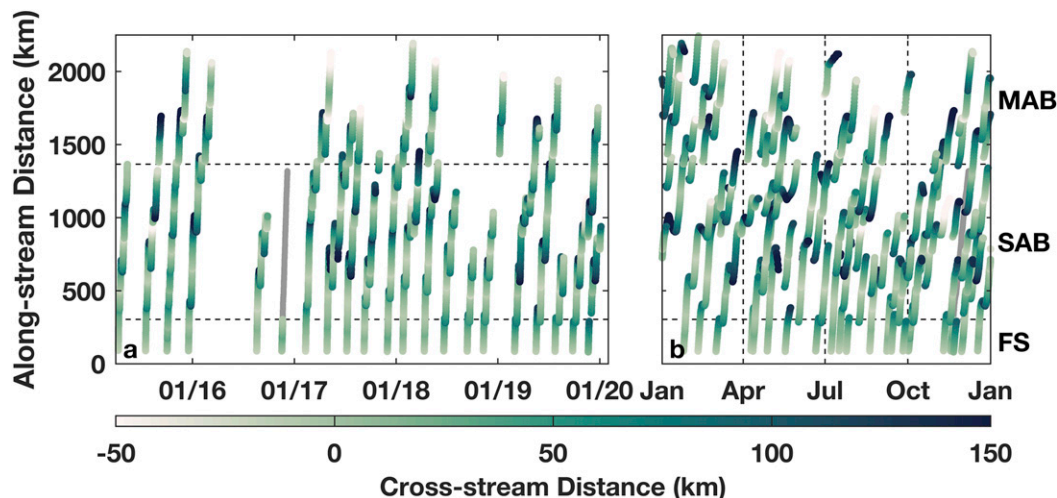
FIG. 2. Spray glider sampling in the Gulf Stream as a function of along-stream distance from 25°N and time. (a) Sampling from Apr 2015 through Jan 2020. (b) All sampling since 2004 as a function of time of year instead of measurement date. Vertical and horizontal dashed lines delineate seasons and dynamical regions (FS, SAB, MAB), respectively. Points are colored by cross-stream position relative to where the 15°C isotherm is found at a depth of 200 m, except for part of one glider mission in late 2016 when the CTD failed (gray).
