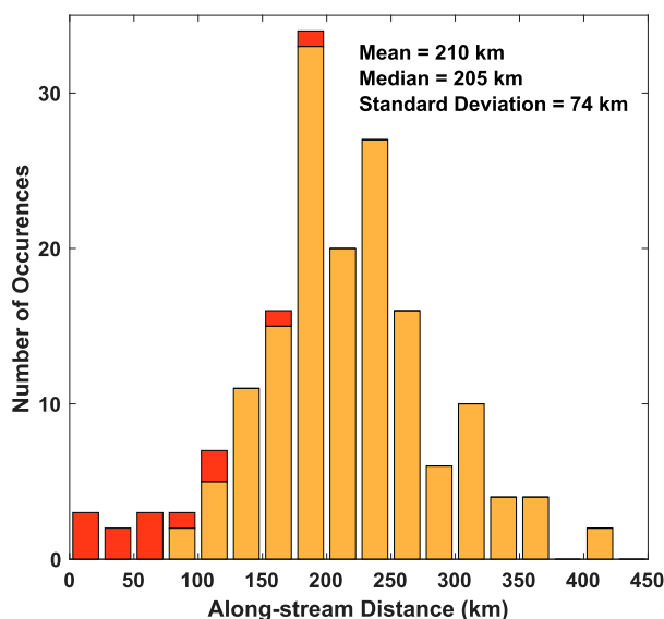
FIG. 6. Histogram of the along-stream distances covered during all glider (orange) and Line W (red) transects that are used for transport calculations. The mean, median, and standard deviation of along-stream extent are given in the upper-right corner.
