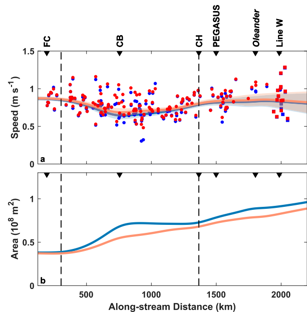
FIG. 12. (a) Transport-weighted speed and (b) inferred Gulf Stream area above 1000m as functions of along-stream distance. Colors, lines, symbols, vertical dashed lines, and location indicators as in Fig. 10. The shading is the standard error of the weighted mean velocity and assumes that all of the error in velocity is due to an error in speed and not direction.
