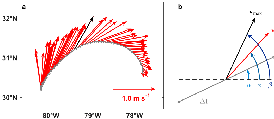
FIG. 7. (a) Example transect from a mission near 31°N during July 2015. Gray line segments correspond to the glider displacements \Delta l during each dive with locations of GPS fixes denoted by crosses. Depth-average currents \mathbf{v}_{DA} for each dive are shown as red arrows. The dive with the maximum transport per unit distance for the entire transect \mathbf{v}_{max} is highlighted in black. A unit arrow is shown for scale in the lower-right corner. (b) Zoomed version of (a) showing only a single glider dive to highlight the vectors and angles used to calculate transport. The vector \mathbf{v} represents the local current, \alpha is the angle of the glider displacement, \phi is the angle of the local current, and \beta is the angle corresponding to \mathbf{v}_{max} . All angles are measured counterclockwise from east.
