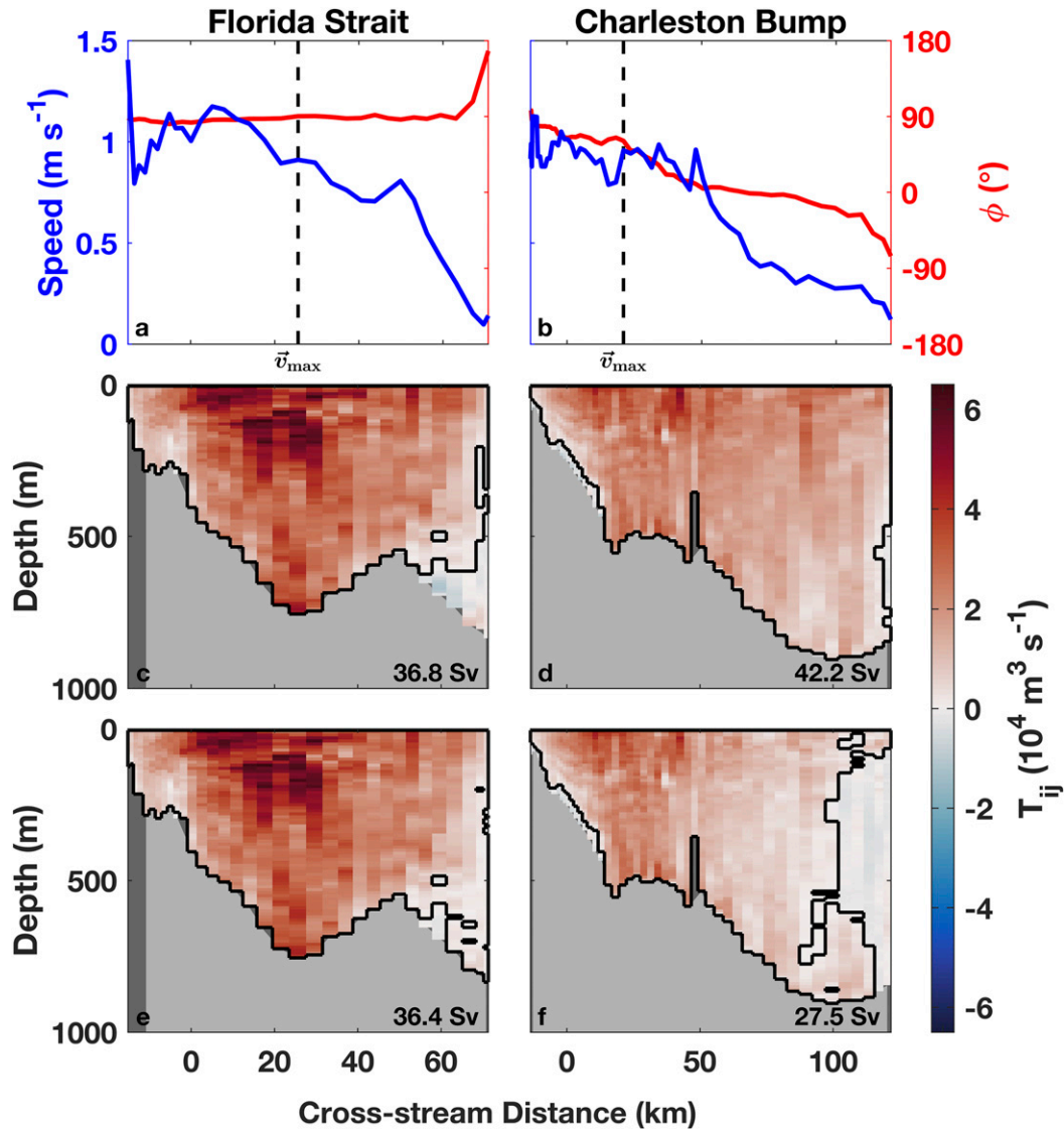
FIG. 9. Two example transects across the Gulf Stream (left) from the Florida Strait and (right) in the vicinity of the Charleston Bump (same transect as shown in Figs. 7 and 8). (a),(b) Speed (blue) and direction clockwise from east ( \phi ; red) of depth-average currents. The location of \vec{v}_{\max} is indicated by dashed vertical black lines. (c),(d) Upper bound of the transport through each cell ( T_{ij,upper} ). (e),(f) lower-bound of the transport through each cell ( T_{ij,lower} ). In (c)–(f), the black line outlines the region of integration for transport calculations. Light gray indicates the bathymetry as measured by the glider’s AD2CP, while regions without data are dark gray. Corresponding volume transport estimates are shown in the lower right of (c)–(f).
