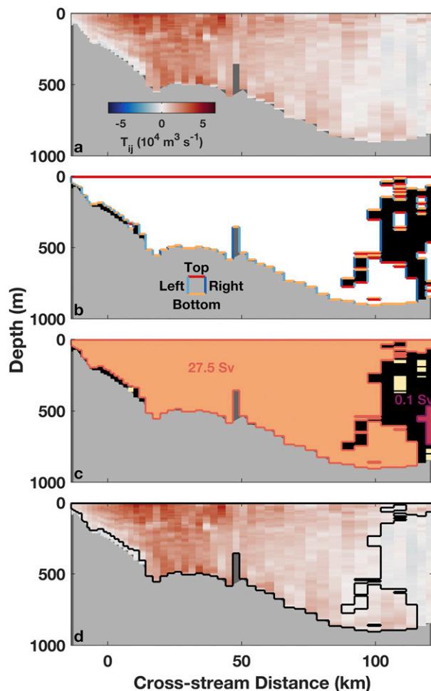
FIG. 8. Step-by-step example illustrating the procedure for determining limits of integration for transport calculations in Eq. (1). The bathymetry as measured by the glider's AD2CP is shaded light gray. Dark gray indicates regions where there are no data. (a) T_{ij,lower} for the transect shown in Fig. 7a. (b) Binary matrix that has value 1 (white) when T_{ij} > 0 and 0 otherwise (black). Top/bottom/left/right edges of regions of positive T_{ij} are drawn in indicated colors. (c) Connected regions of positive T_{ij} and their correspondingly colored edges. The orange region with the largest transport is the Gulf Stream, the magenta region contains the second largest transport. Regions with smaller transports are shown in yellow. As in (b), black indicates regions where T_{ij} is negative. (d) T_{ij} as in (a) with the resulting integration boundary of the Gulf Stream in black.
