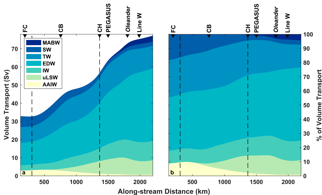
FIG. 14. Along-stream evolution of Gulf Stream volume transport by water class (as defined in Fig. 13) using the upper-bound transport estimates. (a) Stacked area plot of absolute volume transport for each water class. (b) Volume transport by water class as a fraction of the total transport. Vertical dashed lines and triangular tick marks on the upper axes are as in Fig. 10.
