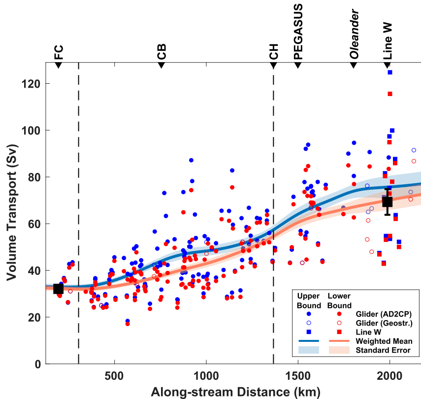
FIG. 10. Gulf Stream volume transport estimates in the upper 1000 m as a function of along-stream distance from 25°N for both the upper and the lower-bound (see legend in the lower right). Individual transport estimates (symbols) are from glider transects across the full width of the Gulf Stream (using either direct velocity measurements from AD2CPs or mapped geostrophic velocities) and from shipboard LADCP casts along Line W. A Gaussian-weighted running mean with 200-km scale (lines) and the bootstrapped standard error of the weighted mean (shading) are shown. Mean volume transport estimates from cable measurements as part of the Western Boundary Time Series in the Florida Strait (Meinen et al. 2010) and from Line W as calculated in Andres et al. (2020) are shown as black squares with whiskers indicating the standard error of the mean. The standard error of \pm 0.2 Sv from Meinen et al. (2010) is too small to be visible. Black triangles on the upper axis indicate the along-stream distances of important geographic locations and sustained transport measurement sites: Florida Cable (FC), Charleston Bump (CB), The Point at Cape Hatteras (CH), PEGASUS line near 73°W, Oleander line, and Line W. The dashed vertical lines distinguish the three different dynamical regions with boundaries as defined in the text: FS, SAB, MAB (from left to right).
