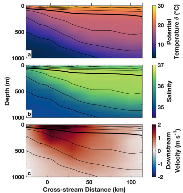
FIG. 5. Example transects of (a) potential temperature \theta , (b) salinity, and (c) downstream velocity in the upper 1000 m from Line W ship-based measurements in May 2013. Tick marks on the upper axes indicate the position of individual CTD/LADCP stations. Isopycnals are as in Fig. 3.
