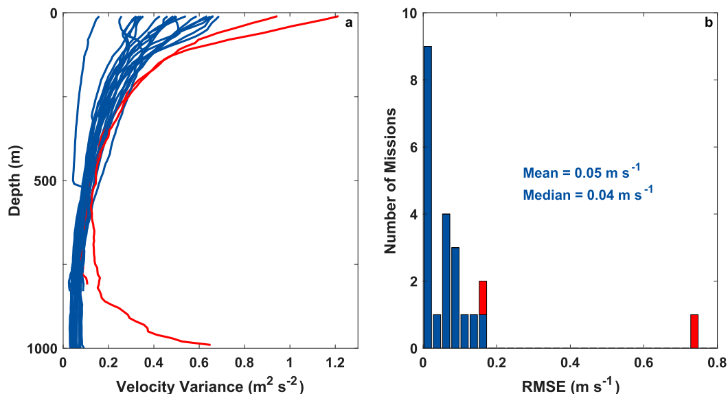
FIG. 4. (a) Vertical profiles of velocity variance for the 22 Gulf Stream glider missions with AD2CPs from the surface to the maximum depth for which at least 40 dives contribute to the variance. Red indicates missions where raw data are not available due to instrument losses. (b) Histogram of the root-mean-square error (RMSE) in velocity profiles for all Gulf Stream missions shown in (a). The mean and median RMSEs for missions with raw data are shown. Color coding is as in (a).
