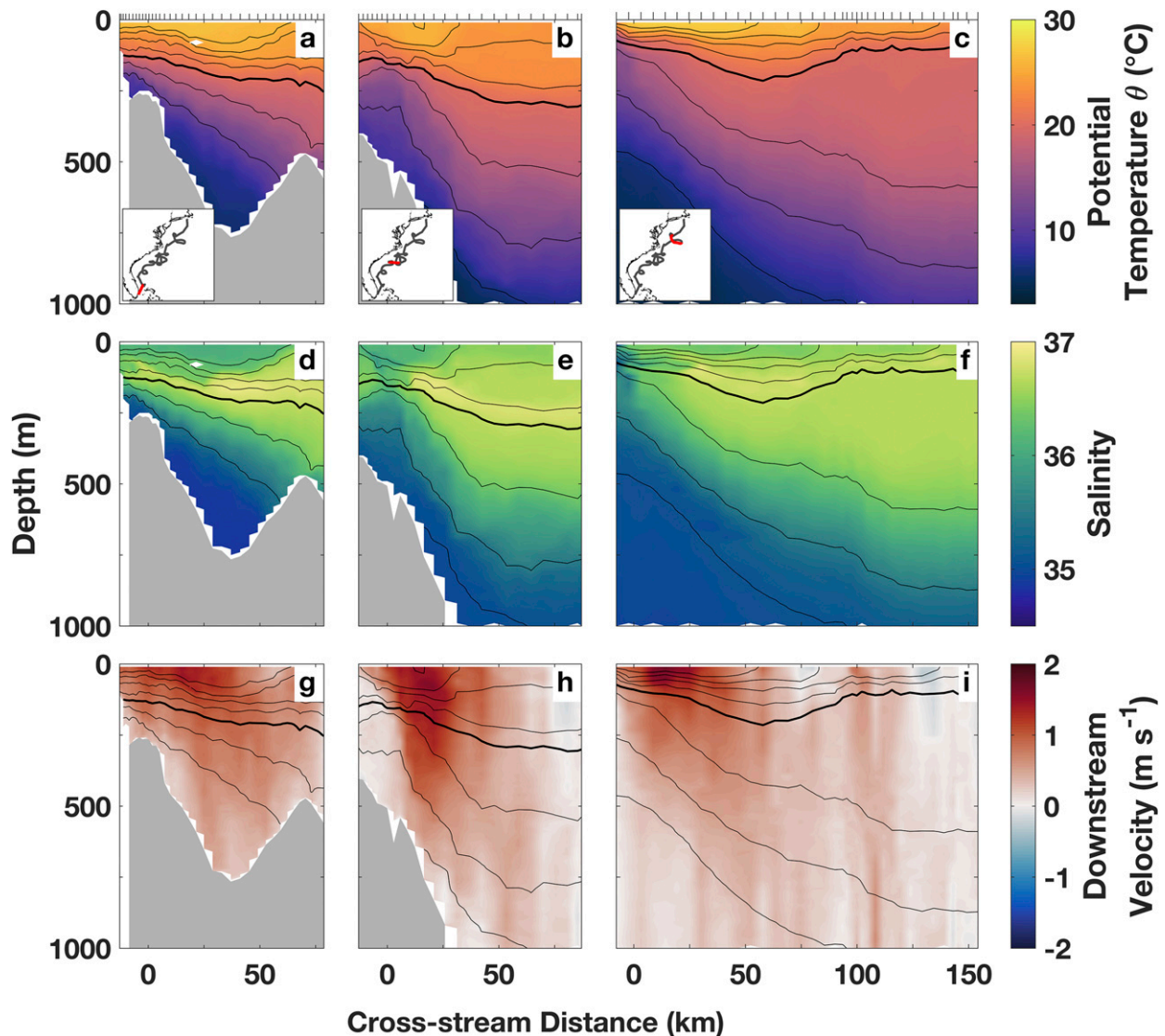
FIG. 3. Example Spray glider transects across the Gulf Stream during spring 2019: (a)–(c) potential temperature \theta , (d)–(f) salinity, and (g)–(i) downstream velocity (i.e., velocity parallel to the measured depth-average current). Black contours are isopycnals with a spacing of 0.5 \text{ kg m}^{-3} and the 26.0 \text{ kg m}^{-3} isopycnal bold. Tick marks on the upper axes indicate the locations of individual profiles. The bathymetry as measured by the glider's AD2CP is shaded gray. From left to right, transects are representative of the FS, SAB, and MAB dynamical regions. Inset maps in (a)–(c) show the location of each transect in red in relation to the complete mission trajectory (gray).
