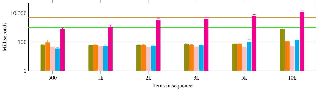
(a) Blazegraph
