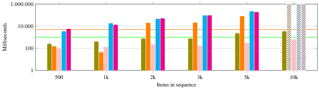
(a) Blazegraph
