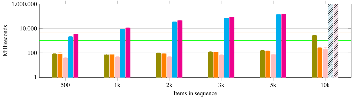
(a) Blazegraph
