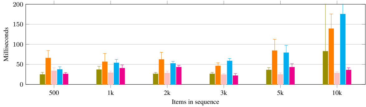
(a) Blazegraph
