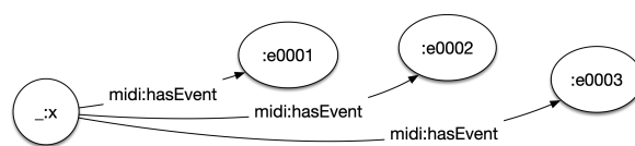
Fig. 2. The URI-based list model. _:x represents the list entity, not necessarily a blank node, linked to all list elements. In this example, the order of the elements is implicit in the tail of the URI, although it could appear before.
