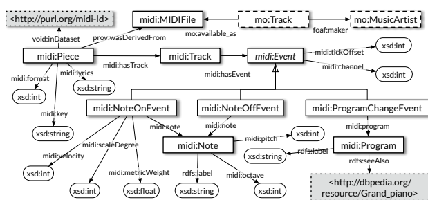
Fig. 7. Excerpt of the MIDI ontology. Tracks contain lists of sequential MIDI events.
