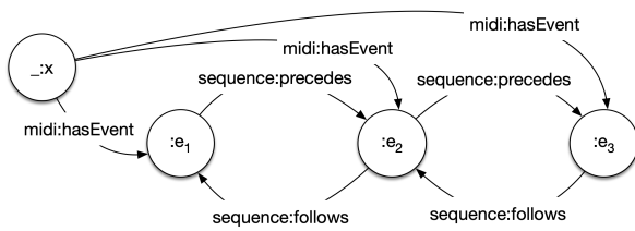
Fig. 4. The Sequence Ontology Pattern model. _:x represents the list entity that connects to list elements through the midi:hasEvent property. The first list element follows no other element, and the last precedes no other element.
