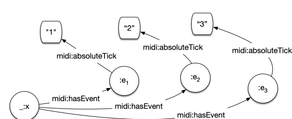
Fig. 3. The Number-based list model. _:x represents the list entity, here connecting to all list elements through a specific midi:hasEvent property that links tracks to events. Order is explicit in each list element through other arbitrary properties (e.g. midi:absoluteTick ).
