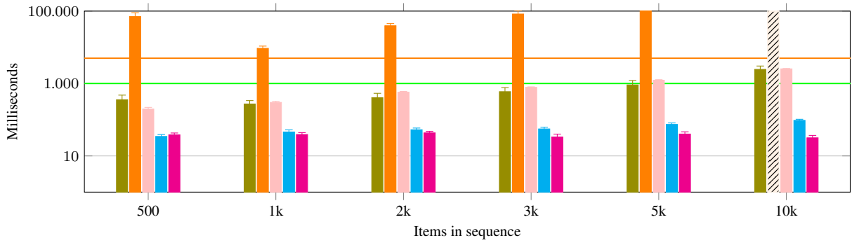
(a) Blazegraph
