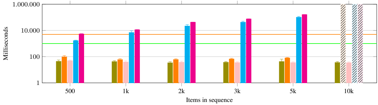
(a) Blazegraph
