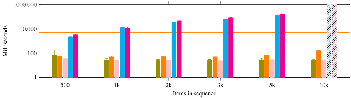
(a) Blazegraph
