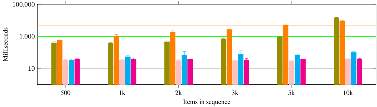
(a) Blazegraph
