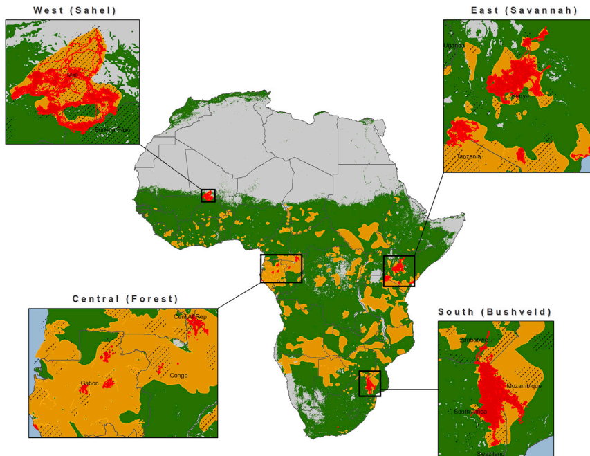
Figure 1. A habitat suitability model for elephants
