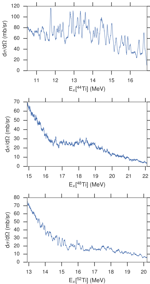
Fig. 1 Measurements of the differential cross-section, made at a centre-of-mass scattering angle of 180°, of the {}^4\text{He}({}^{40}\text{Ca},\alpha) (top), {}^4\text{He}({}^{44}\text{Ca},\alpha) (middle) and {}^4\text{He}({}^{48}\text{Ca},\alpha) (bottom) reactions. The resonances in these measurements are relevant to the structure of {}^{44}\text{Ti} , {}^{48}\text{Ti} and {}^{52}\text{Ti} respectively
