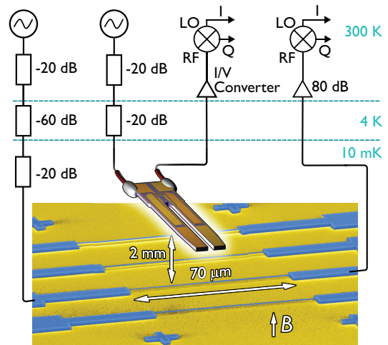
FIG. 1. (Colour online) Schematic of the experimental setup. A tuning fork generates quantum turbulence, whilst a 70 \mu m-long nanomechanical beam, suspended 1 \mu m above the substrate, acts as the detector. The beam and fork are driven by vector network analysers or signal generators through several stages of attenuation at various temperatures. The beam and fork signals are amplified at room temperature by a 80 dB amplifier and an I/V converter 2 . For a detailed description see the Supplementary Information.
