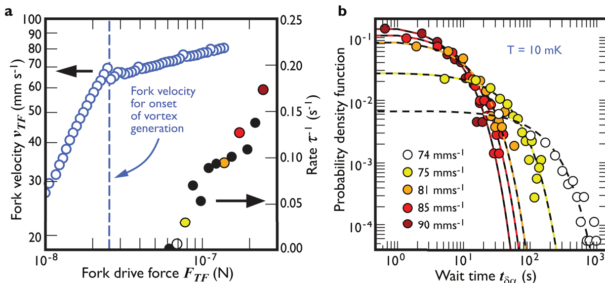
FIG. 3. (Colour online) The capture process. a The tuning fork velocity as a function of the applied force on the left axis and the rate of detected events by the beam on the right axis. The blue circles correspond to the tuning fork force-velocity dependence, while the symbols on the right show the beam detection rate at various fork forces. The dotted blue line corresponds to the onset of turbulence production by the tuning fork. b A probability density function of the wait time between events t_{\delta\alpha} at the same fork velocities. The solid lines correspond to exponential fits, of the form \propto \exp(-t/\tau) . Note symbol colour matching between panels a and b , black points in panel a represent data from other runs not used for panel b . For details, see text.
