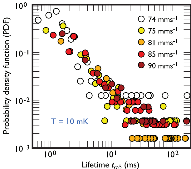
FIG. 4. (Colour online) The release process. A probability density function (PDF) of captured vortex lifetimes t_{\alpha\delta} at selected fork velocities. The discrete data at long lifetimes are the result of single observed events. The data point colours reflect the same data as in Fig. 3.
