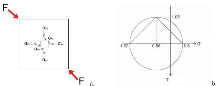
Figure 3: : a. Components of plane stress at panel centroid, b. Graphical interpretation: Mohr's circle (tangential stress ( \tau ), normal stress ( \sigma )) (units in MPa).
