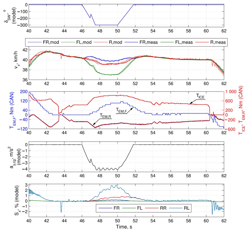
Figure 7. Example of CiL testing results simulating the hybrid powertrain operation when the vehicle negotiates a turn.
