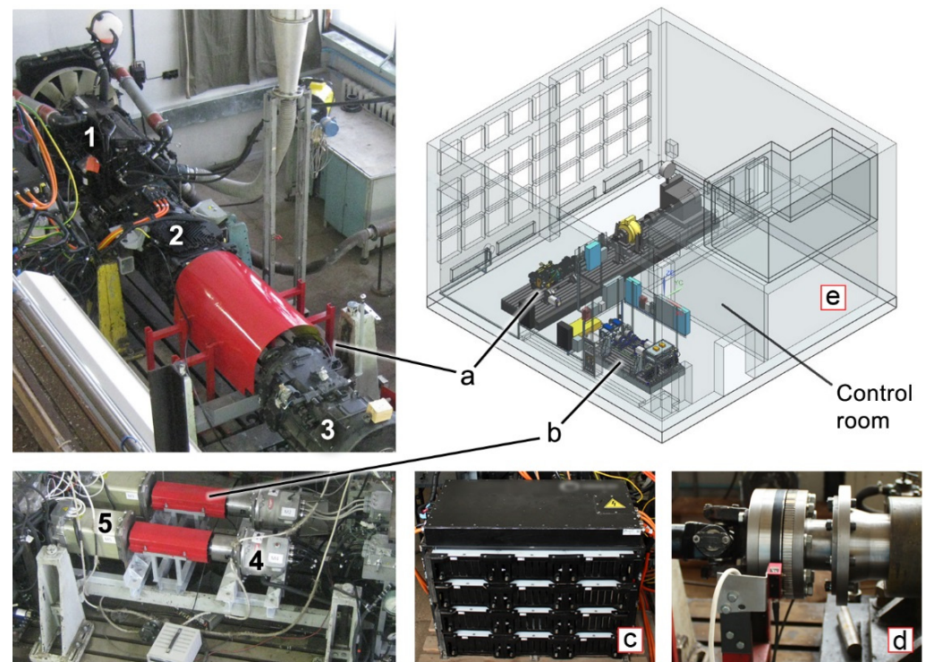
Figure 5. Laboratory setup for CiL testing of the hybrid powertrain. a —test bench for the rear driveline, b —test bench for the front electric drives, c —traction battery, d —torque and rpm sensor installed in the rear driveline’s test bench, e —CAD model of the testing facility. 1—engine, 2—automated gearbox with the hybrid module, 3—loading gearbox, 4—front electric drive, 5—front loading device.
