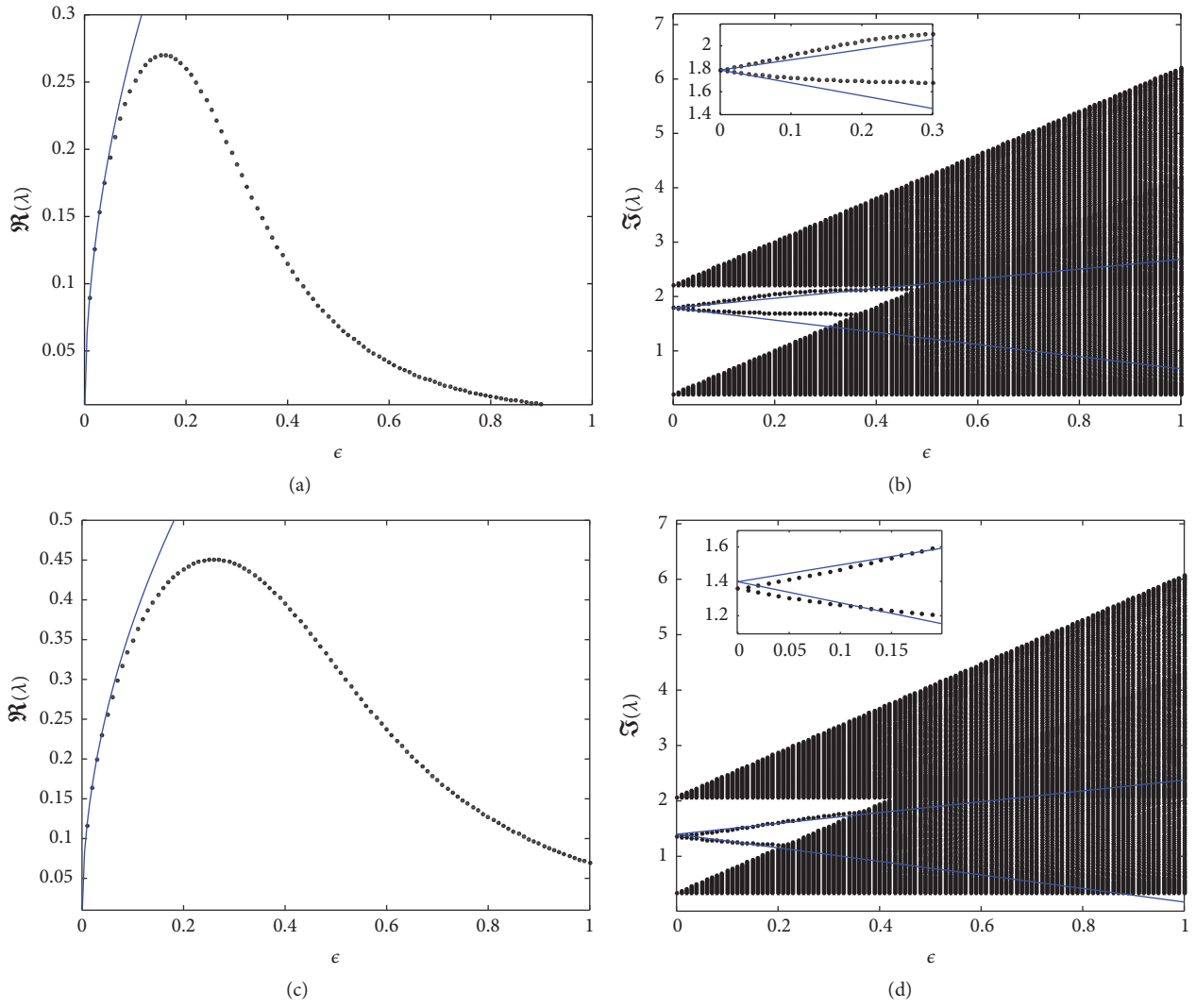
FIGURE 1: Eigenvalues of intersite soliton I with \omega = 1.2, \gamma = 0 (a, b) and 0.5 (c, d). Dots are from the numerics and solid lines are the asymptotic approximations in Section 4.2.1. The collection of dots forming black regions in the right column corresponds to the continuous spectrum.
