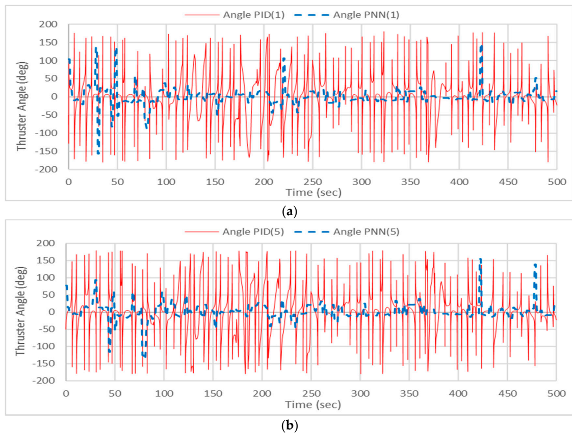
Figure 18. DP simulation with PID and PNN controls showing thruster angle (Head sea): (a) Thruster 1; (b) Thruster 5.
