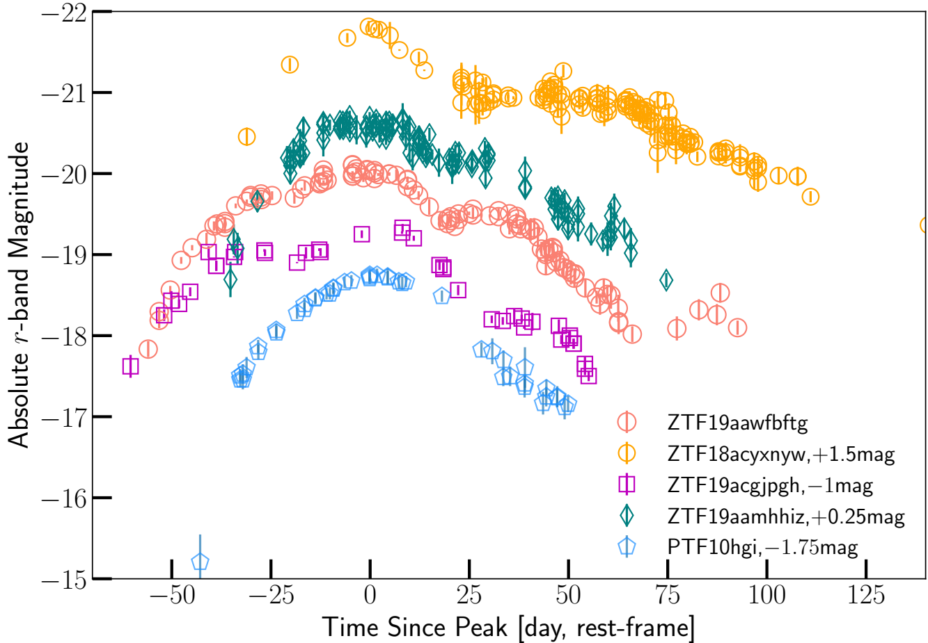
Figure 6. The r -band LCs of the five SLSNe-Ib whose LCs have good phase coverage.
