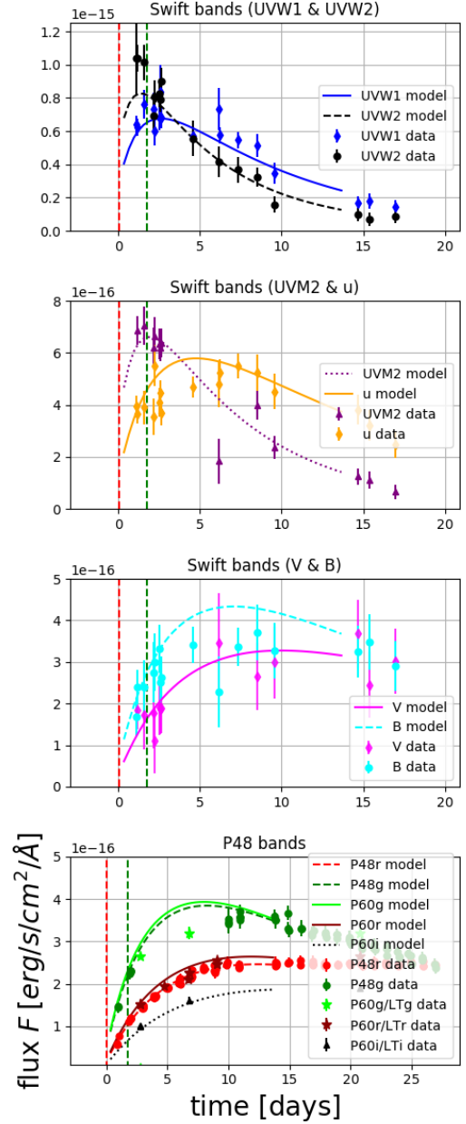
Figure 9. Best fit Morag, Sapir & Waxman model ( \chi^2/dof = 1.69 ) superimposed with the photometric data of SN 2018 fif. The dashed line indicates the lower limit of the temporal validity window for the SW17 (green) and M20 (red) models
