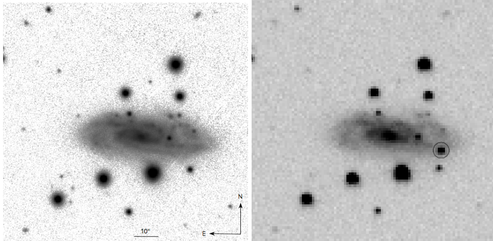
Figure 1. Left panel: the PS1 r -band image b of UGC 85, the host galaxy of the supernova SN 2018 fif. Right panel: the P48 r -band image of SN 2018 fif on September 4 2018, at 9:26:50.00 UT. The circle is centered on the SN position.
