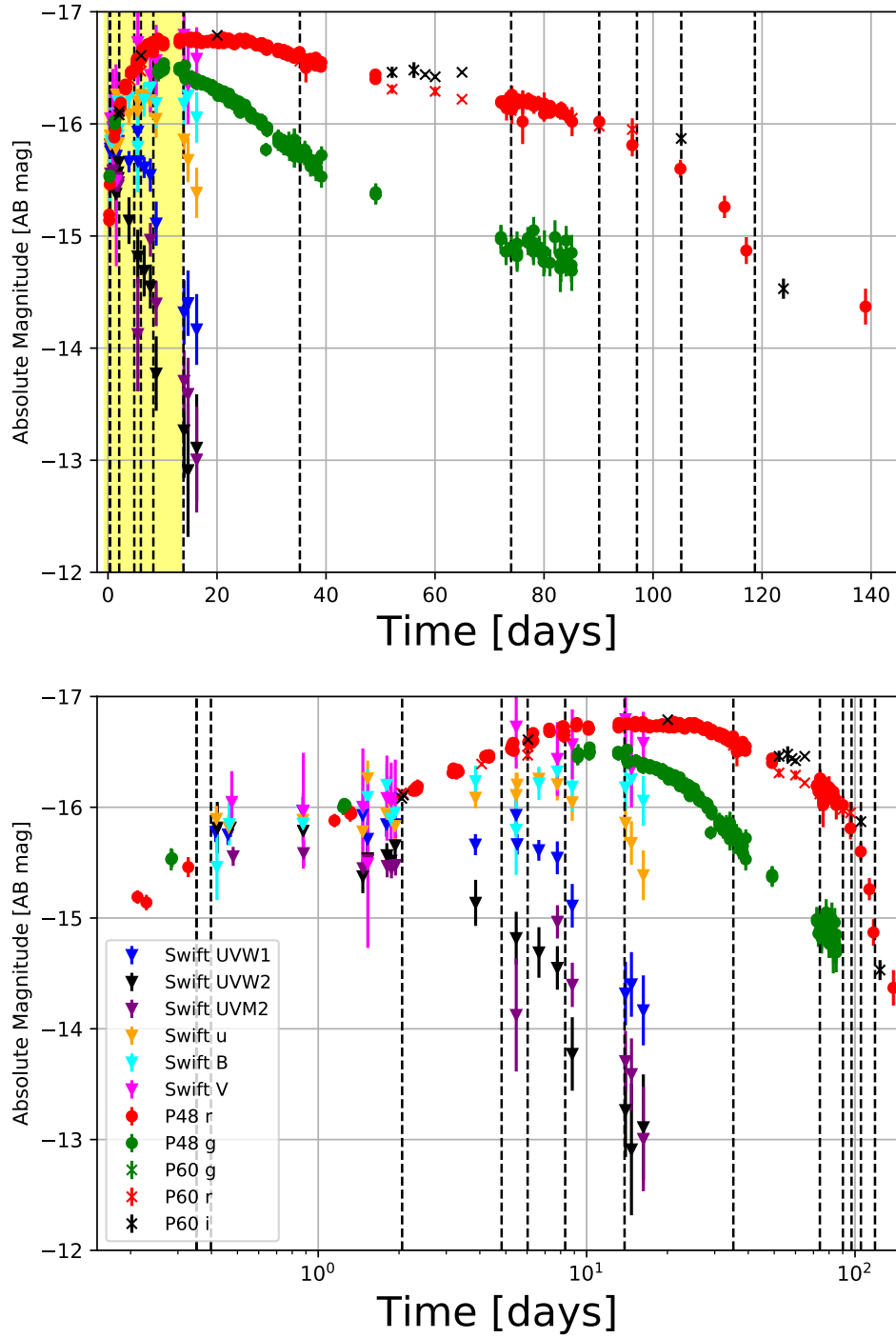
Figure 2. The light curve of SN 2018 fif in linear (top panel) and logarithmic space (lower panel). Time is shown relative to the estimated epoch at which the extrapolated light curve (Equation 1) turns to zero: t_0 = 2458351.6537 , as derived in § 3.1. Black dashed lines indicate dates at which spectroscopic data exist. The yellow background indicates the validity domain of the M20 best fit model: [0.062, 14.107] days relative to the model explosion epoch t_{\text{ref}} , i.e. [-0.641, 13.403] days relative to t_0
