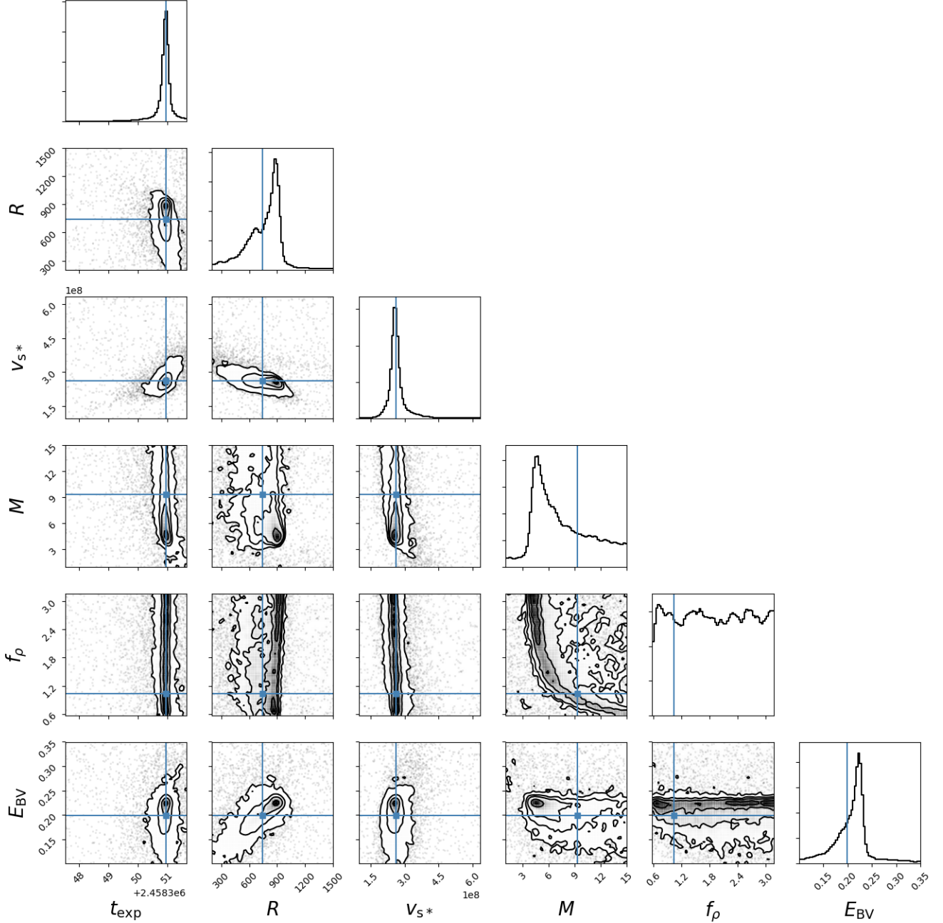
Figure 10. One and two dimensional projections of the posterior probability distributions of the parameters R , v_{s*,8.5} , M , f_{\rho} , t_{\text{ref}} , E_{B-V} , demonstrating the covariance between parameters. The contours correspond to the 1\sigma , 2\sigma and 3\sigma symmetric percentiles. The blue line corresponds to the maximum of the posterior distribution, computed by the dynesty nested sampling algorithm as part of the SOPRANOS-nested package.
