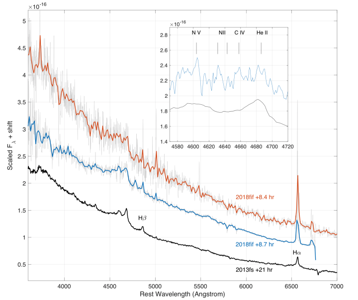
Figure 7. Comparison of early spectra of SN 2018 fif (at 8.4 and 8.7 hr) and SN 2013 fs (at 21 hr; from Yaron et al. 2017). SN 2018 fif shows sharp, narrow Balmer lines lacking a broad electron-scattering base. A broad ledge around 4600 \text{ \AA} indicates a likely blend of weak high-ionization lines, suggesting some CSM emission does exist in this event, though less than in SN 2013 fs, see text.
