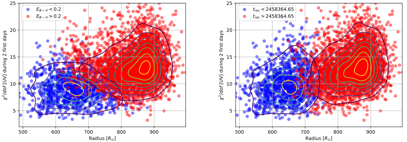
Figure 11. \chi^2/dof of all models in the dynesty chain, considering only the first two days of UV data, as a function of the model progenitor’s radius. The blue and red color coding distinguish between models with different values of (left panel) the extinction and (right panel) the time of recombination. The contours show the density of models. Models (in blue) with E_{B-V} < 0.2 and t_{rec} < 2458364.65 are characterized by smaller radii and a better match the early UV data.
