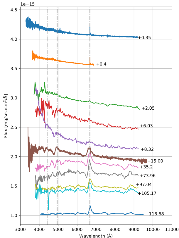
Figure 3. The observed spectra of SN 2018 fif. An offset was applied for easier visualization. Dashed lines indicate the redshifted emission lines for the Balmer series up to H\gamma . The phase is shown relative to the estimated epoch at which the extrapolated r-band light curve (based on Equation 1) turns to zero: t_0 = 2458351.6537 (2018 August 21), as derived in § 3.1.
