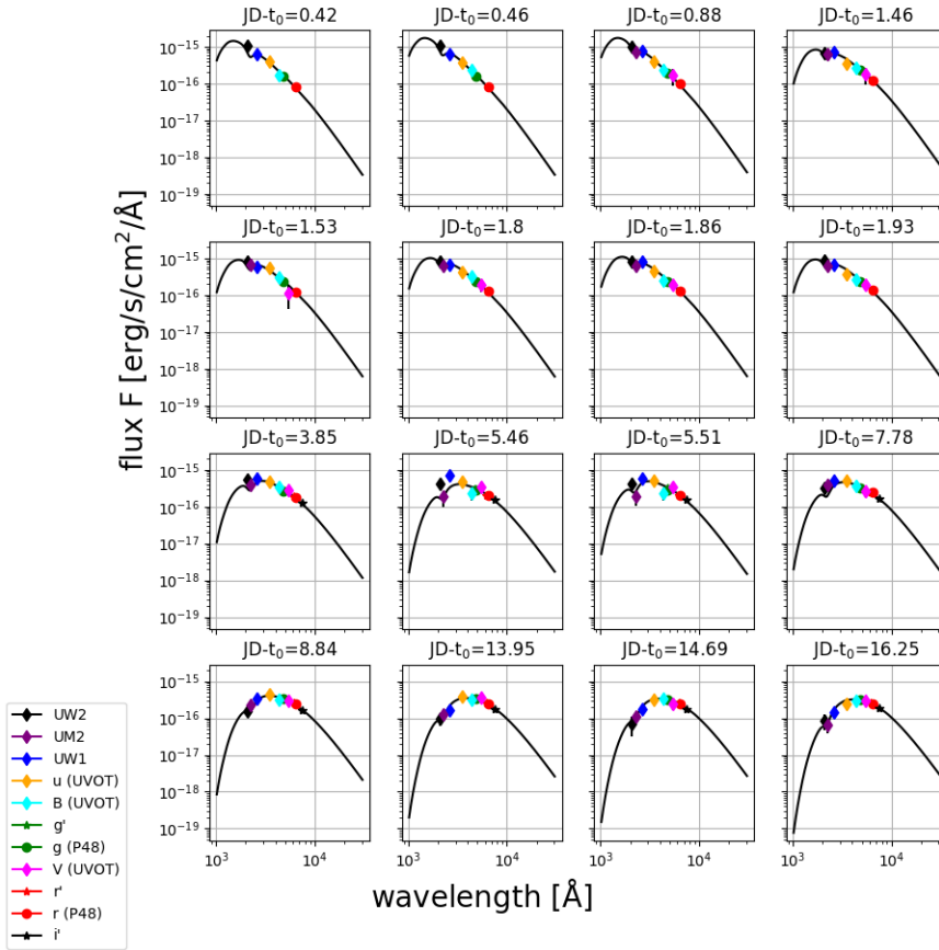
Figure 4. Black body fits to Swift/UVOT and optical photometry for SN 2018fif. Using the PhotoFit tool (released in the appendix), photometric points were interpolated to a common epoch (UVOT epochs), and the errors at the interpolated points were computed with Monte Carlo Markov-chain simulations.
