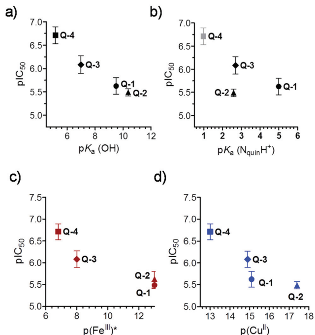
Fig. 6 Correlations between pIC 50 values measured in MES-SA/Dx5 cell lines (IC 50 : mol L -1 ) and pK a (OH) (a), pK a (N quinolinium H + ) (b), pFe(III)* (c) and pCu(II) (d) of the studied 8-hydroxyquinolines. Data are taken from Tables 1 and 2 and Scheme 2.
