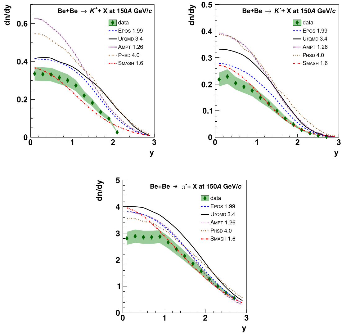
Fig. 35 Comparison of the K^+ (left), K^- (right) and \pi^- (bottom) rapidity spectra for the 20% most central Be+Be collisions at 150A GeV/c with models: EPOS 1.99 (blue dashed line), UrQMD 3.4
