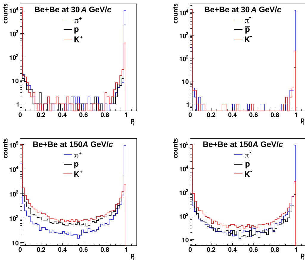
Fig. 14 Probability of a track being a pion, kaon, proton for positively (left) and negatively (right) charged particles from tof - dE/dx measurements in PSD selected Be+Be collisions at 30A (top) and 150A GeV/c (bottom)
