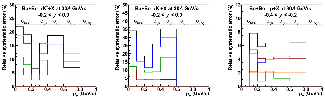
Fig. 18 Contributions to the systematic uncertainty of particle spectra obtained from the tof-dE/dx method at 30A GeV/c as a function of p_T for the rapidity interval -0.2 to 0.0 GeV/c ( K^+ and K^- ) and -0.4 to -0.2 GeV/c (protons). \sigma_{(i)} (red lines) refers to event selection \sigma_{(ii)} (green lines) to the track selection procedure, \sigma_{(iii)} (blue lines) to the
