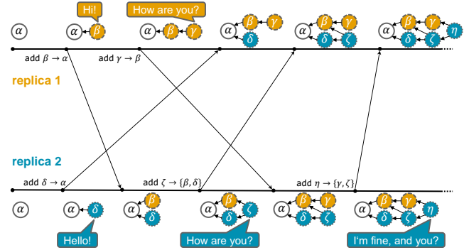
FIGURE 1. Basic example of a MEG and its evolution over time. Two MEG replicas start with an initial state, i.e. a root vertex \alpha . The replica timelines run from left to right, and the replicas’ current DAG state is shown over time. Both replicas concurrently append new vertices to the current state, as indicated by \text{add new vertex} \rightarrow \text{parent vertices} . While the operation is immediately applied to the local state, the arrow from the operation to the other replica represents the delay until the operation is applied on the remote replica. In the chat use case, every new vertex corresponds to a text message, shown by a chat bubble adjacent to the vertex. Replica 1 starts with adding vertices \beta and \gamma in a row, before receiving anything from replica 2. Replica 2 adds vertex \delta concurrently to the addition of \beta . In contrast, vertex \zeta is added after \beta is received, and therefore vertex \zeta gets both \beta and \delta as parent. After vertices \gamma and \zeta have been eventually received, convergence is reached momentarily. Due to the concurrent additions, the number of forward extremities has increased to two. Then, replica 2 adds vertex \eta without concurrent additions from replica 1, which brings the number of forward extremities back to one, and convergence is reached again.
