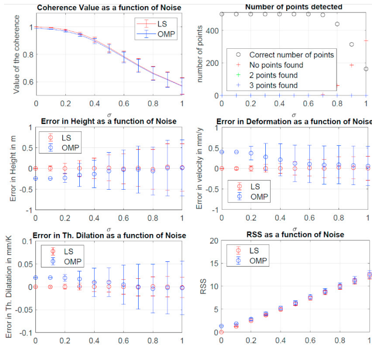
Figure 3: Analysis of the algorithm applied to the first case with only a single PS.
