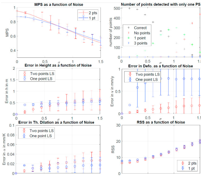
Figure 5: Analysis of the algorithm, applied to the third case with two PS
