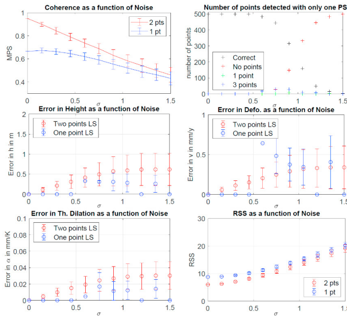
Figure 4: Analysis of the algorithm, applied to the second case with two PS
