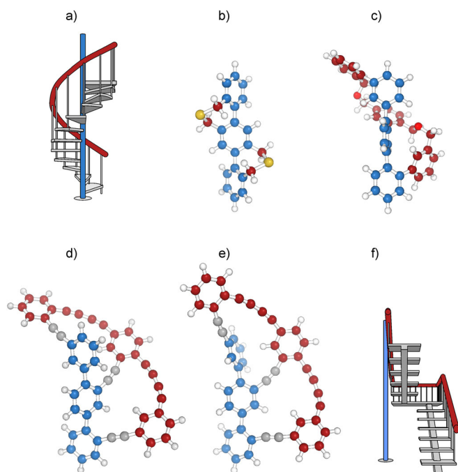
Figure 1. The helical chiral “Geländer” molecules discussed, together with the types of staircases inspiring their design. The structures representing the central axes are blue, and the ones representing the banisters are brick red. a) Spiral staircase. b) The pioneering “Geländer” oligomer described by Vögtle and co-workers. [12] c) Our initial “Geländer” design avoiding achiral meso -forms. [14–16] d) The intended helical arrangement of the 1,4-bis(phenylbuta-1,3-diyn-1-yl) benzene oligomer in our reported target structure 1 . e) The observed spatial arrangement of the 1,4-bis(phenylbuta-1,3-diyn-1-yl) benzene oligomer of 1 according to NMR analyses, resembling rather the banister of a staircase as sketched in f) with an inserted floor.
