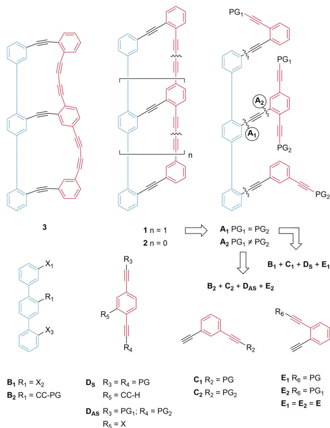
Scheme 1. Chemical structures of the series of macrocyclic oligomers 1 and 2 , together with the retrosynthetic considerations for the assembly of 1 from the building blocks B–E .
