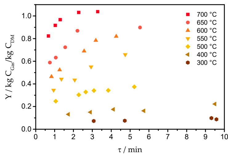
Figure 4. Carbon gasification yield (Y) as a function of the mean residence time ( \tau ) in the hot reaction section of the reactor at different temperatures. Corn silage, 5 wt.% dry matter (DM). Original data available in [43].
