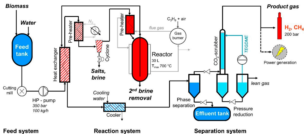
Figure 1. Simplified scheme of the VERENA (acronym for the German expression “experimental facility for the energetic exploitation of agricultural matter”) pilot plant (one-stream process configuration). Adapted from [37].
