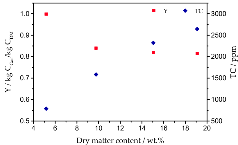
Figure 3. Carbon gasification yield (Y) and total carbon (TC) in the reactor effluent as a function of the dry matter content of the feed slurry (corn silage). Reaction temperature 700 °C, pressure 250 bar. Original data available in [43].
