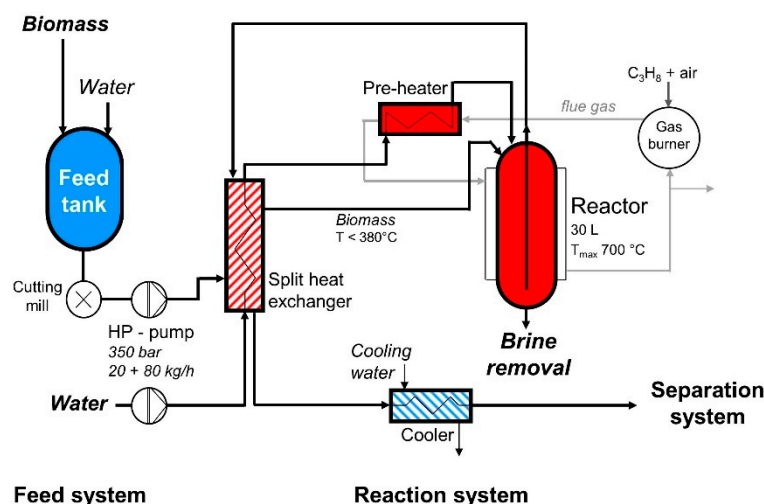
Figure 2. Two-stream process configuration: simplified scheme of the feed and reaction system. Adapted from [38].
