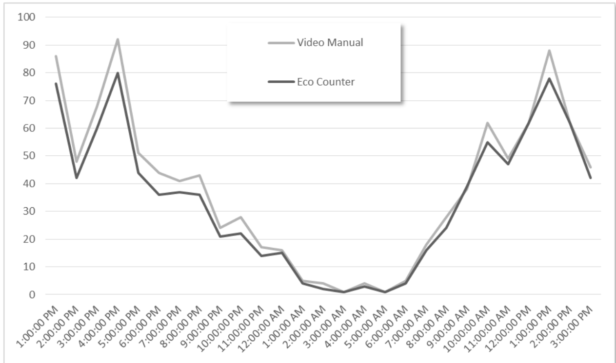
Figure 34. Video-based manual and EcoCounter count comparison.
