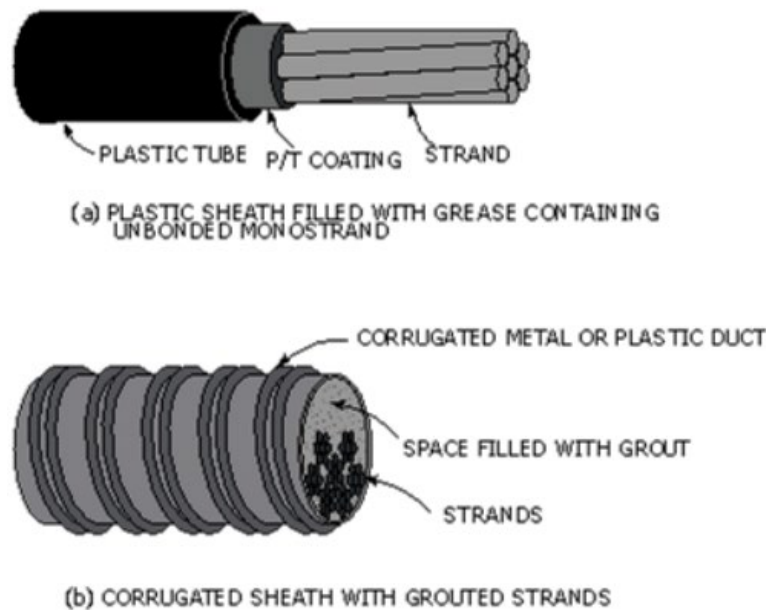
Figure 2.3: Post-tensioning strands (typical) (a) unbonded post-tensioning strand and (b) bonded post-tensioning strand (Vejvoda, 2018)
