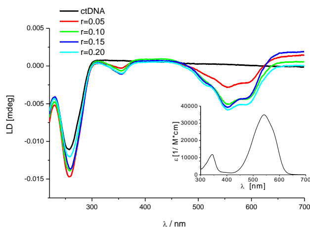
Figure 4. Changes in the flow–linear dichroism (LD) spectra of calf thymus DNA (ct-DNA) ( c = 2 \times 10^{-4} mol·dm -3 ) at various ratios r = [\text{F1}]/[\text{ct-DNA}] . The induced negative signal in the LD spectra corresponds to the absorption band of F1, the inset shows F1 UV/vis absorption spectrum.
