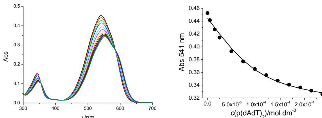
Figure 1. Changes in UV/Vis spectrum of compound F1 ( c = 1 \times 10^{-5} \text{ mol}\cdot\text{dm}^{-3} ) upon titration with poly dAdT–poly dAdT (LEFT) and dependence of absorbance at \lambda_{\text{max}} = 541 \text{ nm} on (poly dAdT–poly dAdT), pH 5.0, sodium cacodylate buffer, I = 0.05 \text{ mol}\cdot\text{dm}^{-3} (RIGHT). The fitting to the Scatchard eq [29,30] (-) yielded parameters shown in Table 2.
