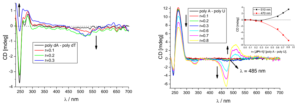
Figure 3. Changes in the circular dichroism (CD) spectra of poly dA–poly dT (LEFT, c = 2 \times 10^{-5} mol·dm -3 ) and poly A–poly U (RIGHT, c = 2 \times 10^{-5} mol·dm -3 ) upon the addition of F1 in various ratios r = [\text{F1}]/[\text{polynucleotide}] .
