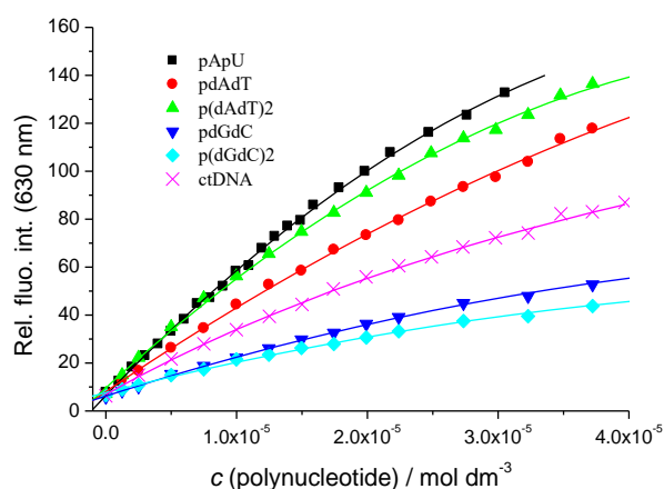
Figure 2. Strong increase of emission intensity of F1 ( c = 1 \times 10^{-5} \text{ mol}\cdot\text{dm}^{-3} , \lambda_{\text{exc.}} = 541 \text{ nm} ) at \lambda_{\text{em.}} = 630 \text{ nm} upon the addition of various ds-polynucleotides (sodium cacodylate buffer, pH = 5.0, I = 0.05 \text{ mol}\cdot\text{dm}^{-3} ). Data were fitted by non-linear least square procedure according the Scatchard equation [29,30] (-) and results are given in Table 2.
